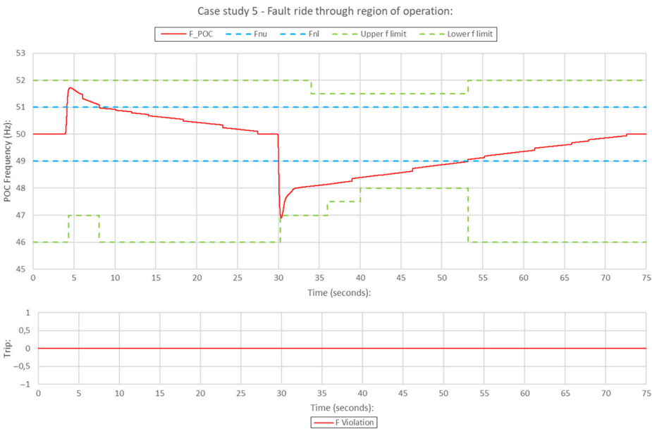
Figure 9. Case study 5, fault ride-through real-time results
