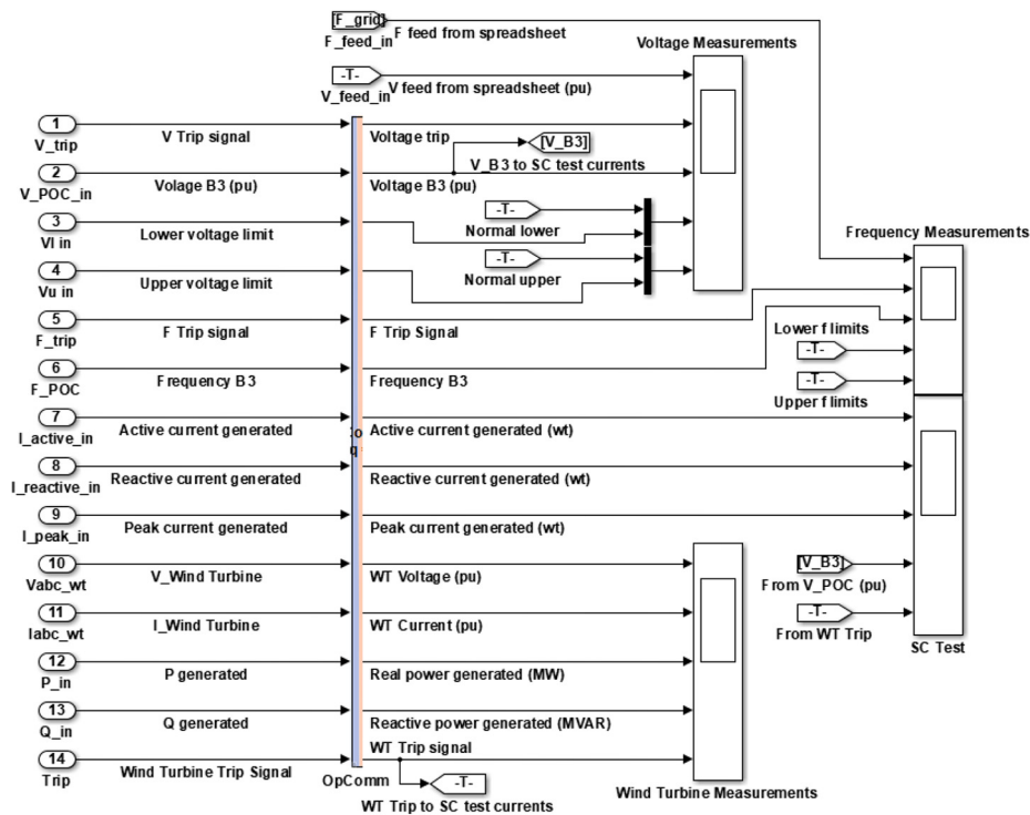
Figure 4. Testbed measurement scopes
