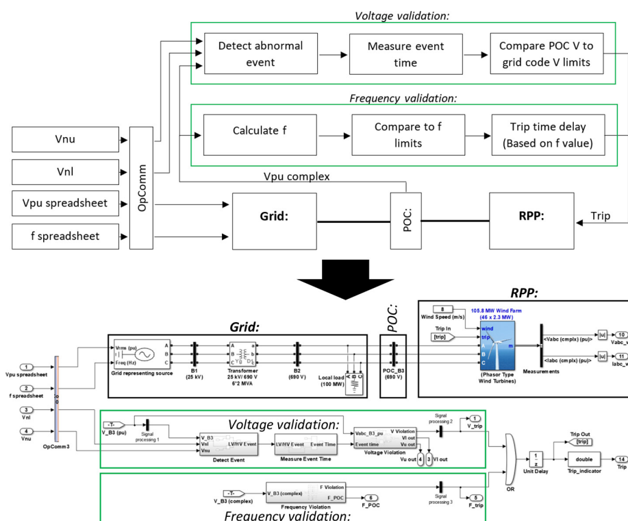
Figure 3. MATLAB SM target sub-system flow diagram and circuit
