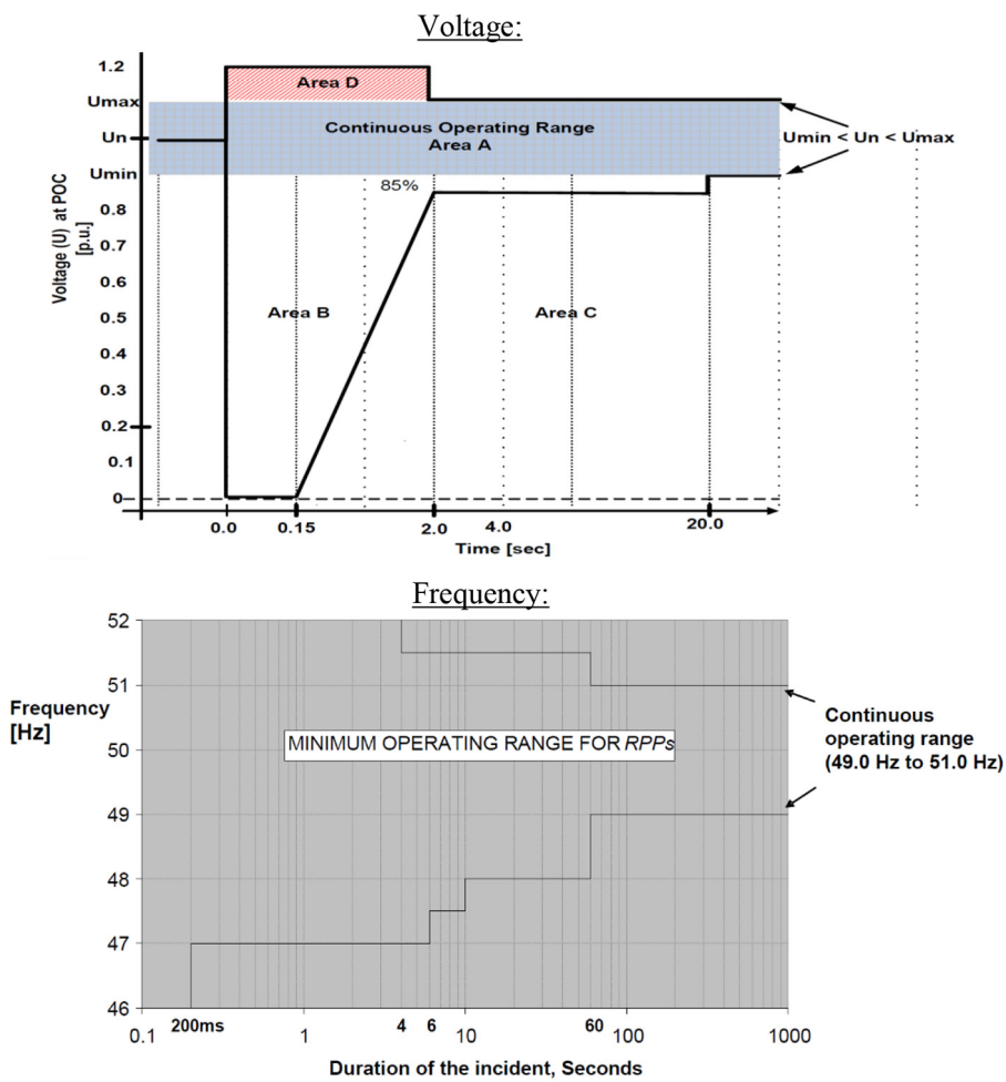
Figure 1. Non-synchronous Category C RPP voltage and frequency ride- through requirements
