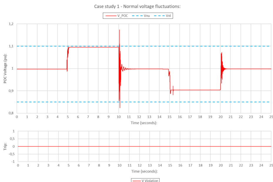
Figure 5. Case study 1, normal voltage fluctuations real-time results
