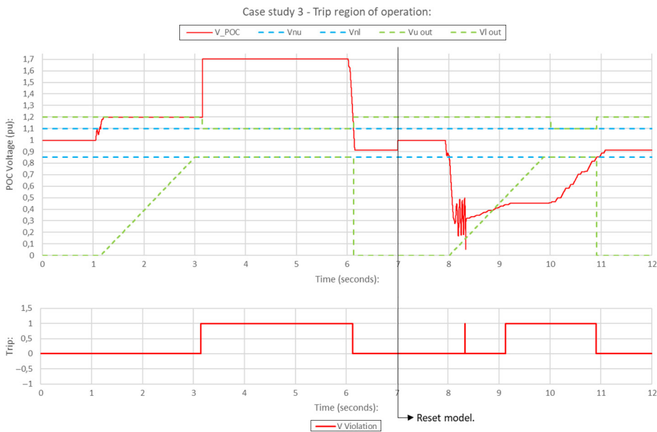
Figure 7. Case study 3, trip region real-time results
