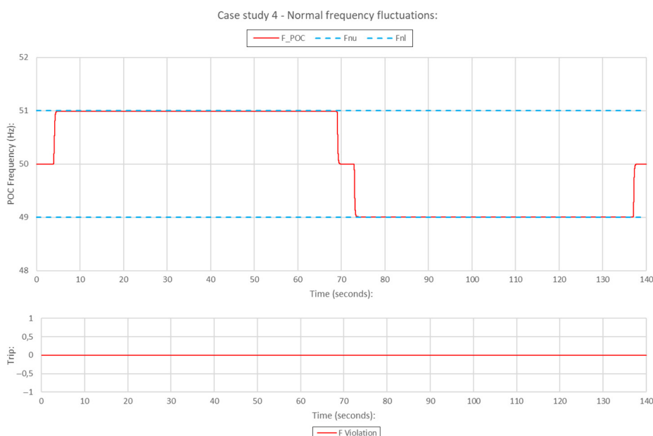
Figure 8. Case study 4, normal frequency fluctuations real-time results
