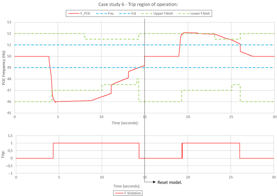
Figure 10. Case study 6, trip region real-time results
