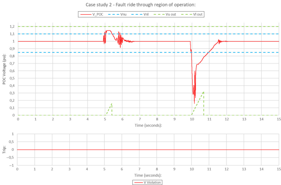
Figure 6. Case study 2, fault ride-through real-time results
