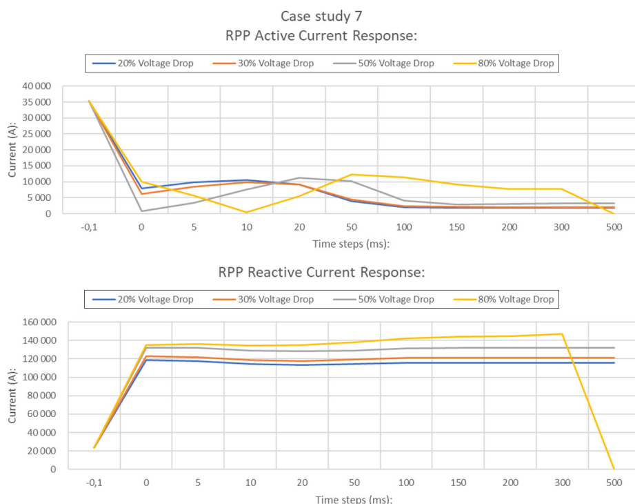
Figure 11. Case study 7, RPP active and reactive current response
