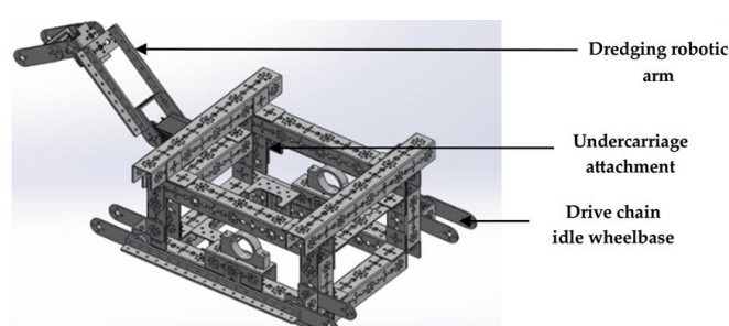
Figure 3—Framework for undercarriage design
