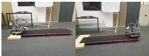
Figure 12—Drive test experiment for EPRSDC at an angle of 0°
