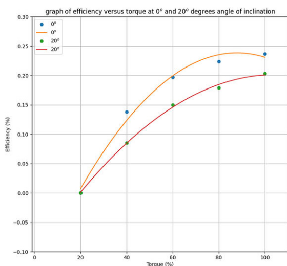
Figure 24—Graph of efficiency versus torque at 0° and 20° angles of inclination
