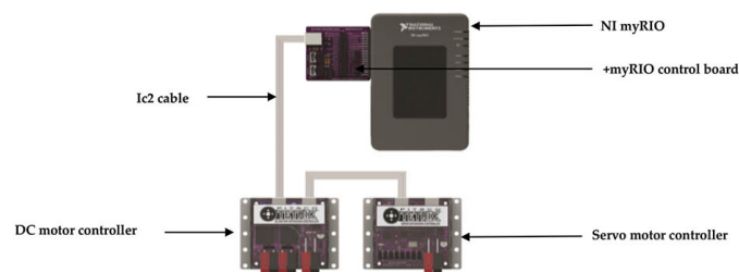
Figure 6—Electric powered robotic subsea crawler
