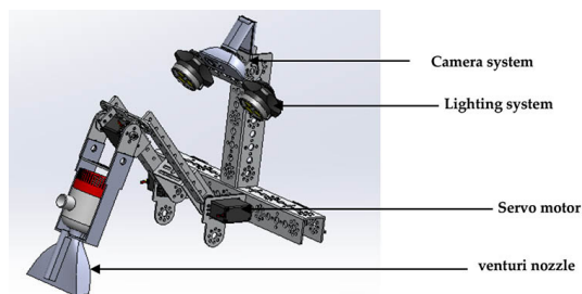
Figure 4—Two-degree-of-freedom boom arm with a venturi dredging nozzle
