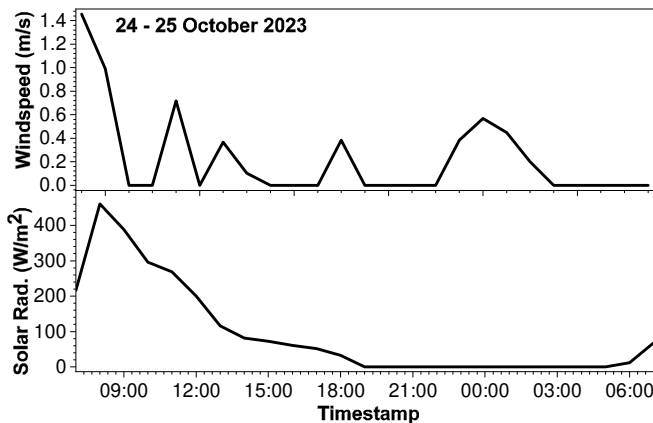
Fig. 17. Solar irradiance and wind speed vs time (day 8).
