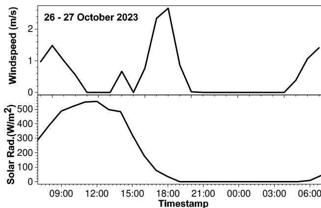
Fig. 18. Solar irradiance and wind speed vs time (day 10).
