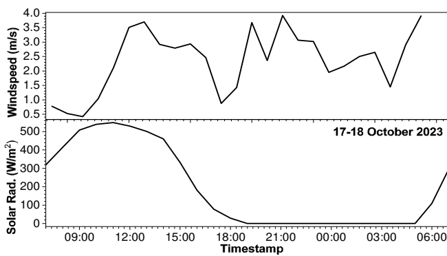
Fig. 6. Solar irradiance and wind speed vs time (day 1).
