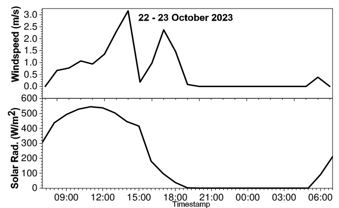
Fig. 11. Solar irradiance and wind speed vs time (day 6).
