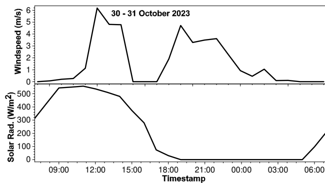
Fig. 8. Solar irradiance and wind speed vs time (day 11).
