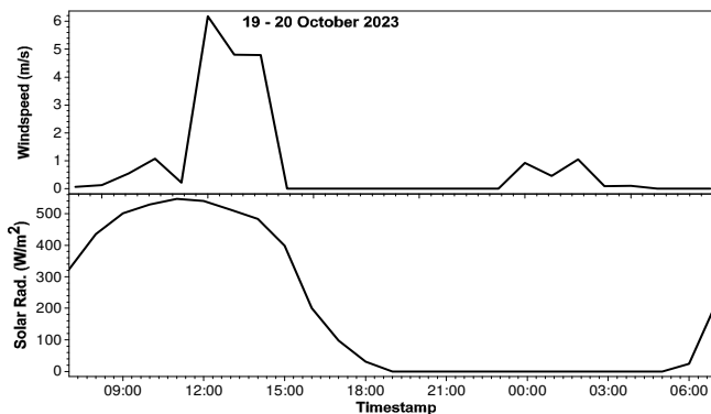
Fig. 7. Solar irradiance and wind speed vs time (day 3).
