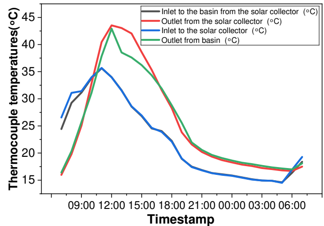
Fig. 14. Thermocouple temperatures vs timestamp.
