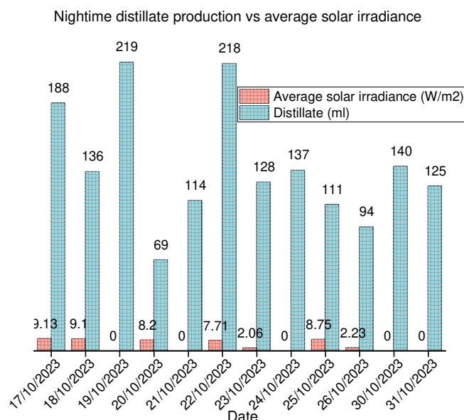
Fig. 21. Night time distillate production vs average solar irradiance.
