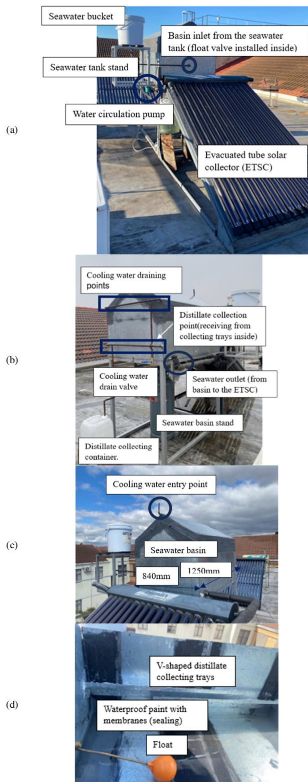
Fig. 1. Solar still (a) overview including the ESTC, (b) seawater piping, (c) basin measurements, (d) inside the water basin.
