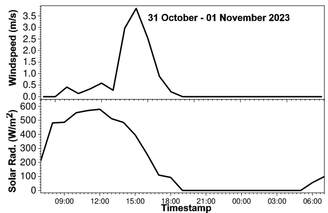
Fig. 9. Solar irradiance and wind speed vs time (day 12).
