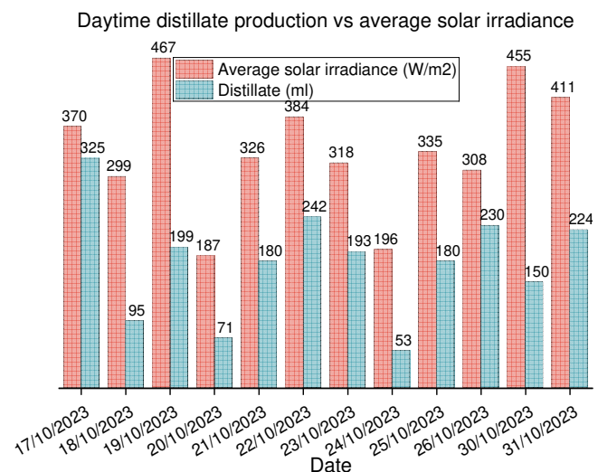
Fig. 19. Day time distillate production vs average solar irradiance.
