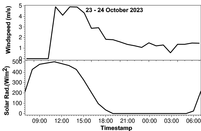
Fig. 12. Solar irradiance and wind speed vs time (day 7).
