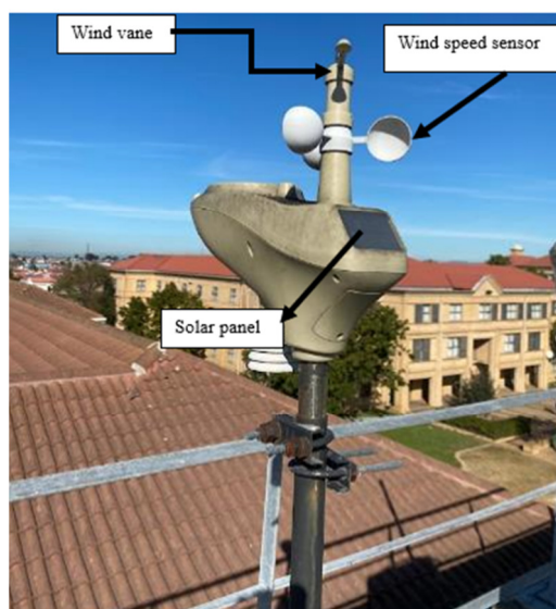
Fig. 2. HP2000 wireless weather station.
