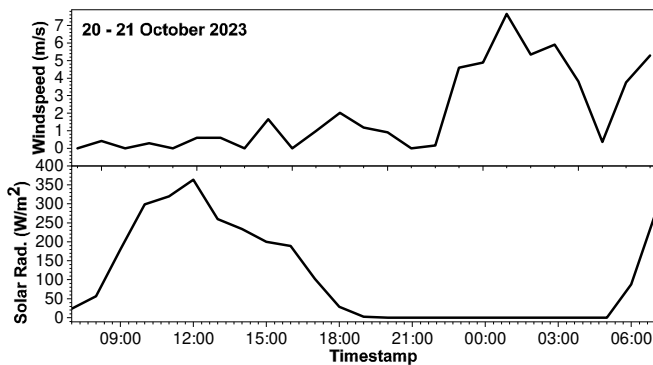
Fig. 16. Solar irradiance and wind speed vs time (day 4).
