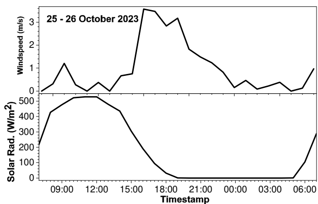
Fig. 13. Solar irradiance and wind speed vs time (day 9).
