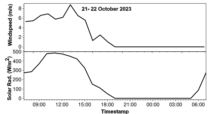
Fig. 10. Solar irradiance and wind speed vs time (day 5).
