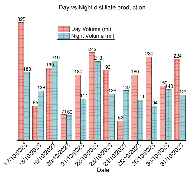
Fig. 22. Day and night distillate production.
