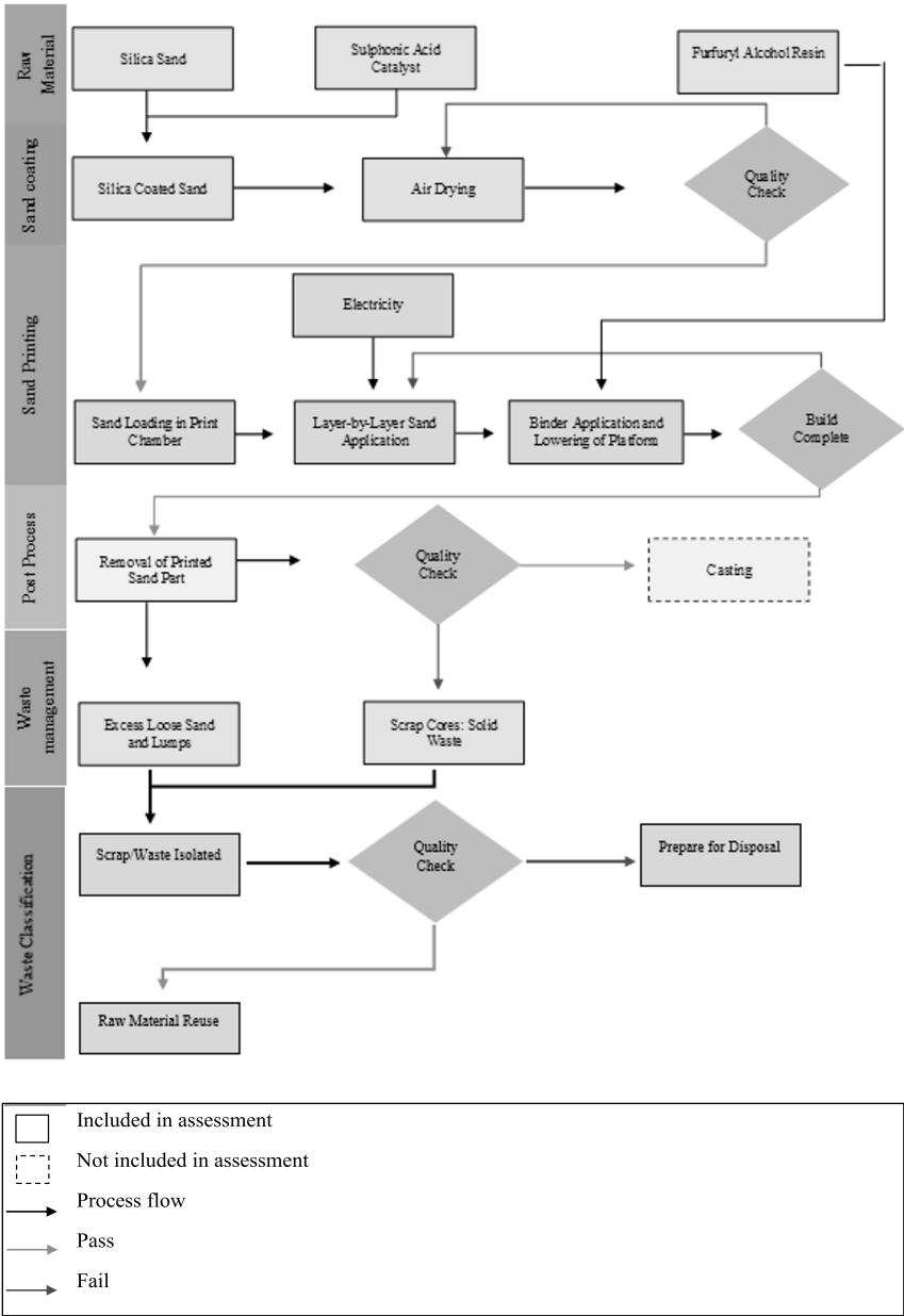
Fig. 4. System boundary of assessment for the 3D sand printing process.
