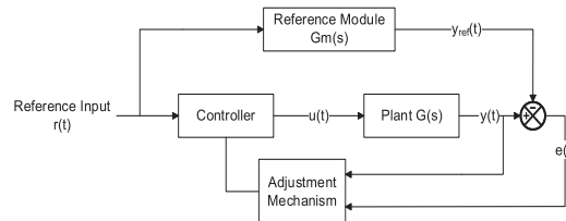
Fig. 2. MRAC system, [7]
