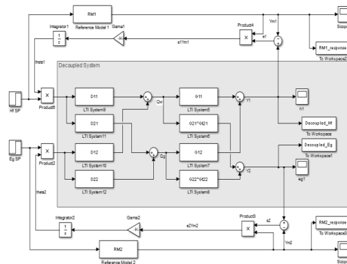
Fig. 3. Simulink Model of Decoupled MRAC of a flotation process
