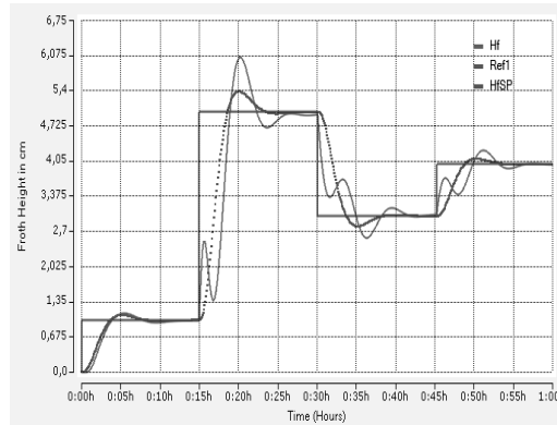
Fig. 7. Real-time simulation results of Froth Height with respect to time
