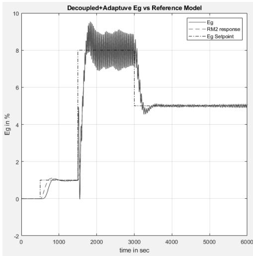
Fig. 6. Gas Holdup Simulation Set-point Tracking
