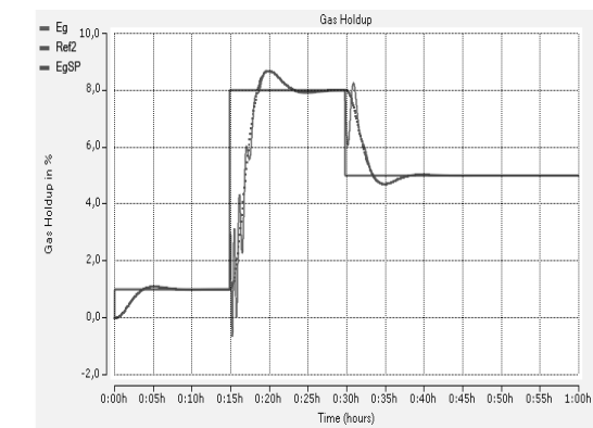
Fig. 8. Real-time simulation results of Gas Holdup with respect to time
