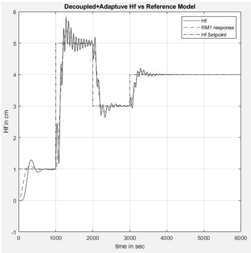
Fig. 5. Froth Height Simulation Set-point Tracking
