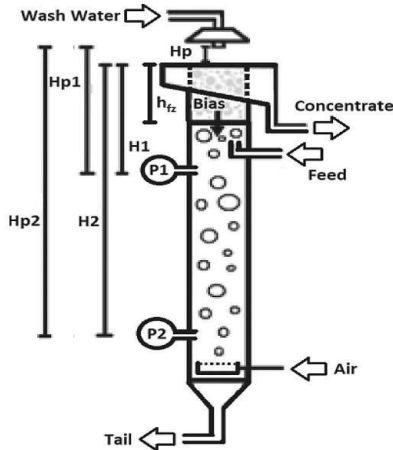
Fig. 1. Pilot Flotation Column, [3]
