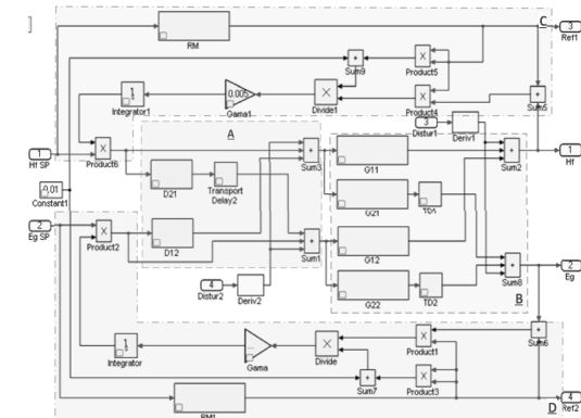
Fig. 4. TwinCAT3 Decoupled MRAC of a Flotation Process
