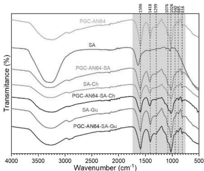
Figure 1. ATR-FTIR spectra of PGC-AN64-SA, PGC-AN64-SA-Ch, PGC-AN64-SA-Gu beads, and PGC-AN64 from Aspergillus niger strain HO32. PGC-AN64-SA: PGC-AN64 immobilized with sodium alginate, PGC-AN64-SA-Ch: PGC-AN64 immobilized with sodium alginate and chitosan, PGC-AN64-SA-Gu: PGC-AN64 immobilized with sodium alginate and guar gum. The ATR-FTIR profile was generated by OriginLab OriginPro software 2021b (SR1).
