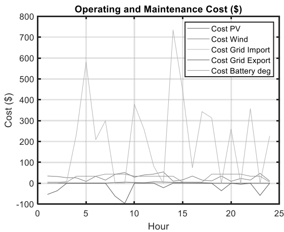
Figure 8. Operating and Maintenance cost results for 24 hours using GWO
