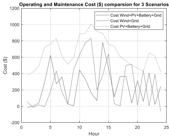
Figure 12. Operating and Maintenance cost Comparison for 3 Scenarios
