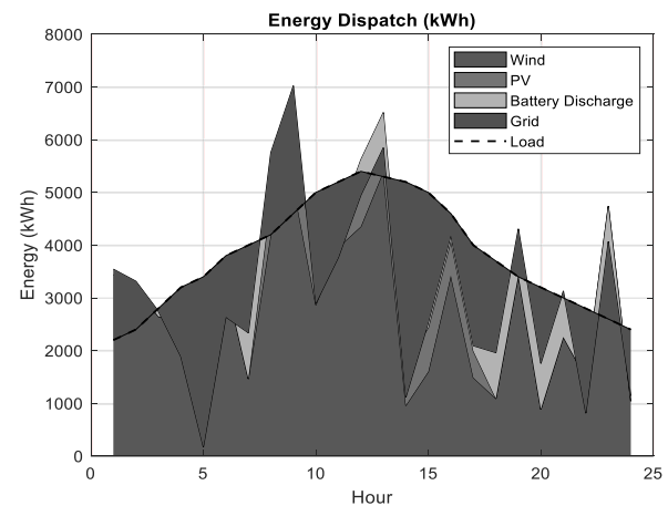
Figure 7. Energy Dispatch simulation results for 24 hours using GWO
