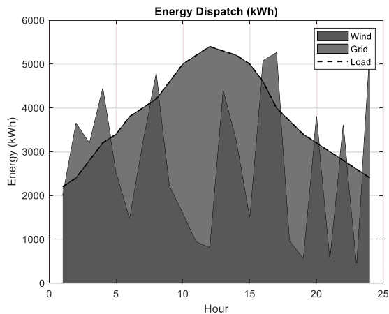
Figure 9. Energy Dispatch simulation results for 24 hours using GWO
