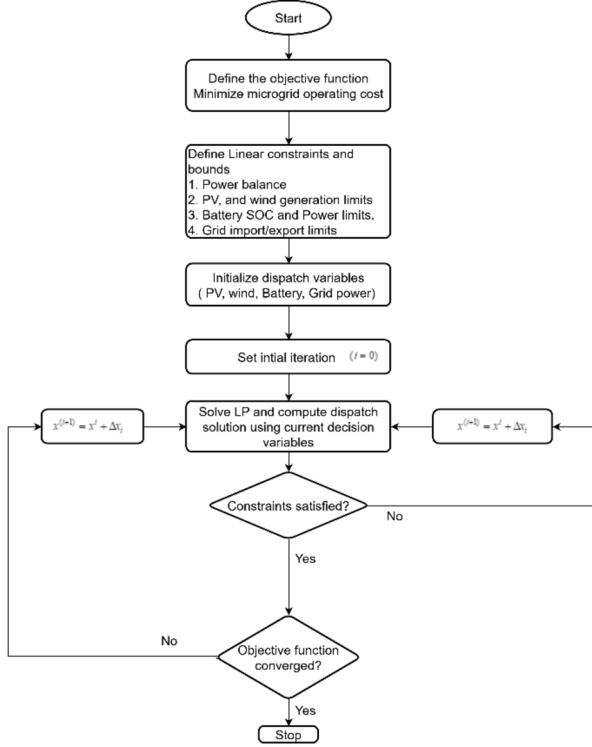
Figure 1. Flow chart for Linear Programming Optimization
