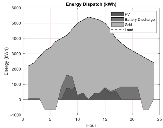
Figure 11. Energy Dispatch for 24 hours using GWO
