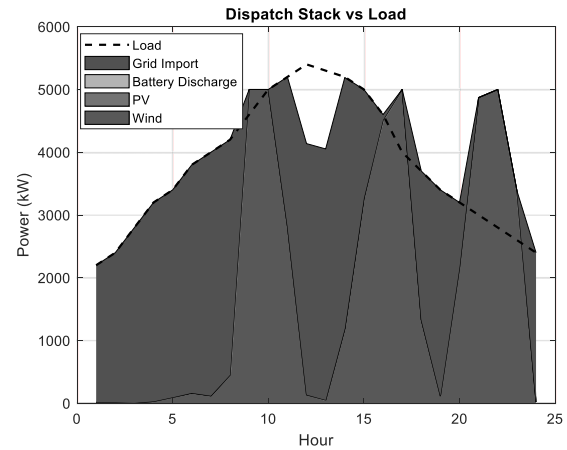
Figure 5. Grid-connected Microgrid dispatch with Wind Energy for 24 hours using LP
