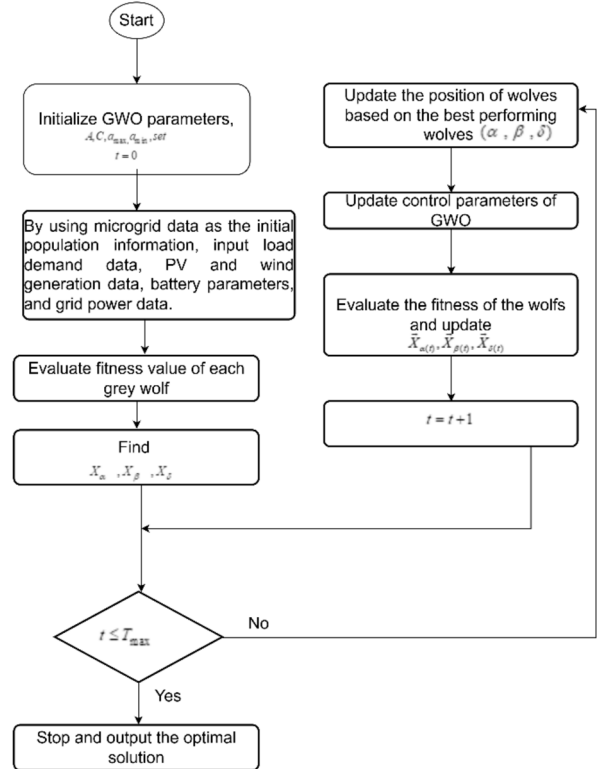
Figure 2. Flowchart of the Grey Wolf Optimization Algorithm for Grid-connected Microgrid dispatch using Wind, PV, and Battery
