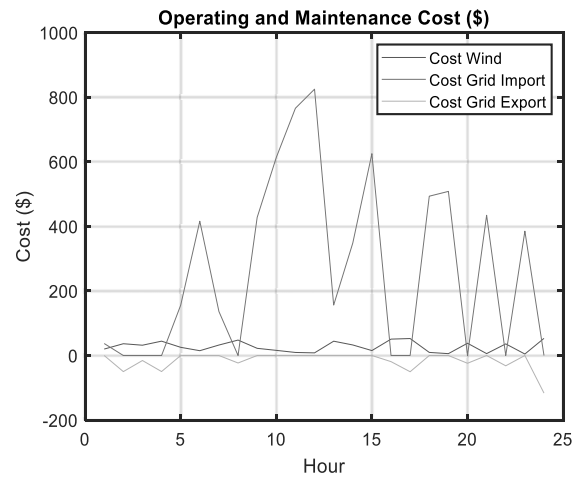
Figure 10. Operating and maintenance cost for 24 hours using GWO
