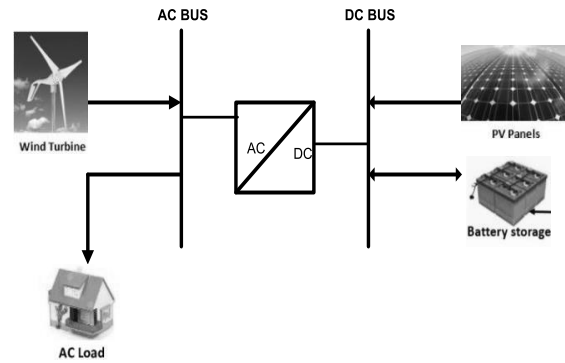
Figure 3. Single-line diagram of the proposed Microgrid network
