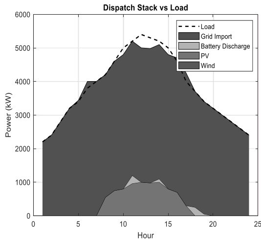
Figure 6. Grid-connected Microgrid dispatch with PV and Battery results for 24 hours using LP
