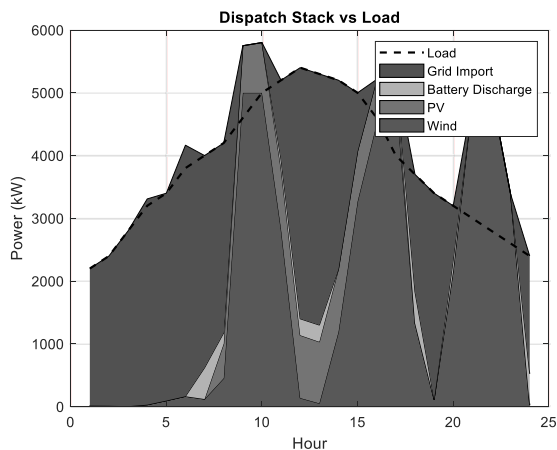
Figure 4. Grid-connected Microgrid dispatch with Wind, PV, and Battery using LP algorithm for 24 hours
