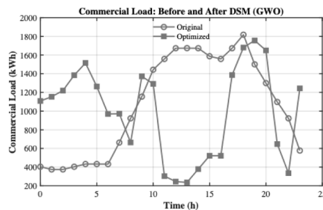
Fig 7. Commercial Load Results Before and After Grey Wolf Optimization
