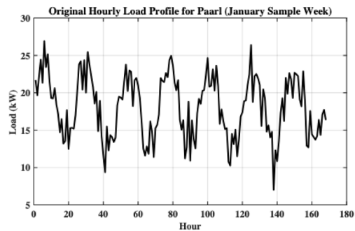
Fig 5: Original Hourly Load Profile for large user customer in Paarl (January 2025 Sample Week)
