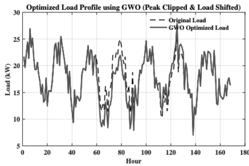
Fig 4: Optimized Load Profile using GWO (Peak Clipping &amp; Load Shifting)
