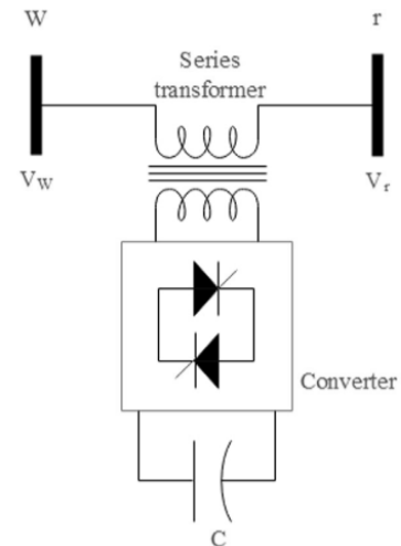
Fig. 2. Static synchronous series compensator circuit [23].
