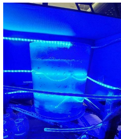
Fig. 2 30 L bubble column used for microalgae cultivation
