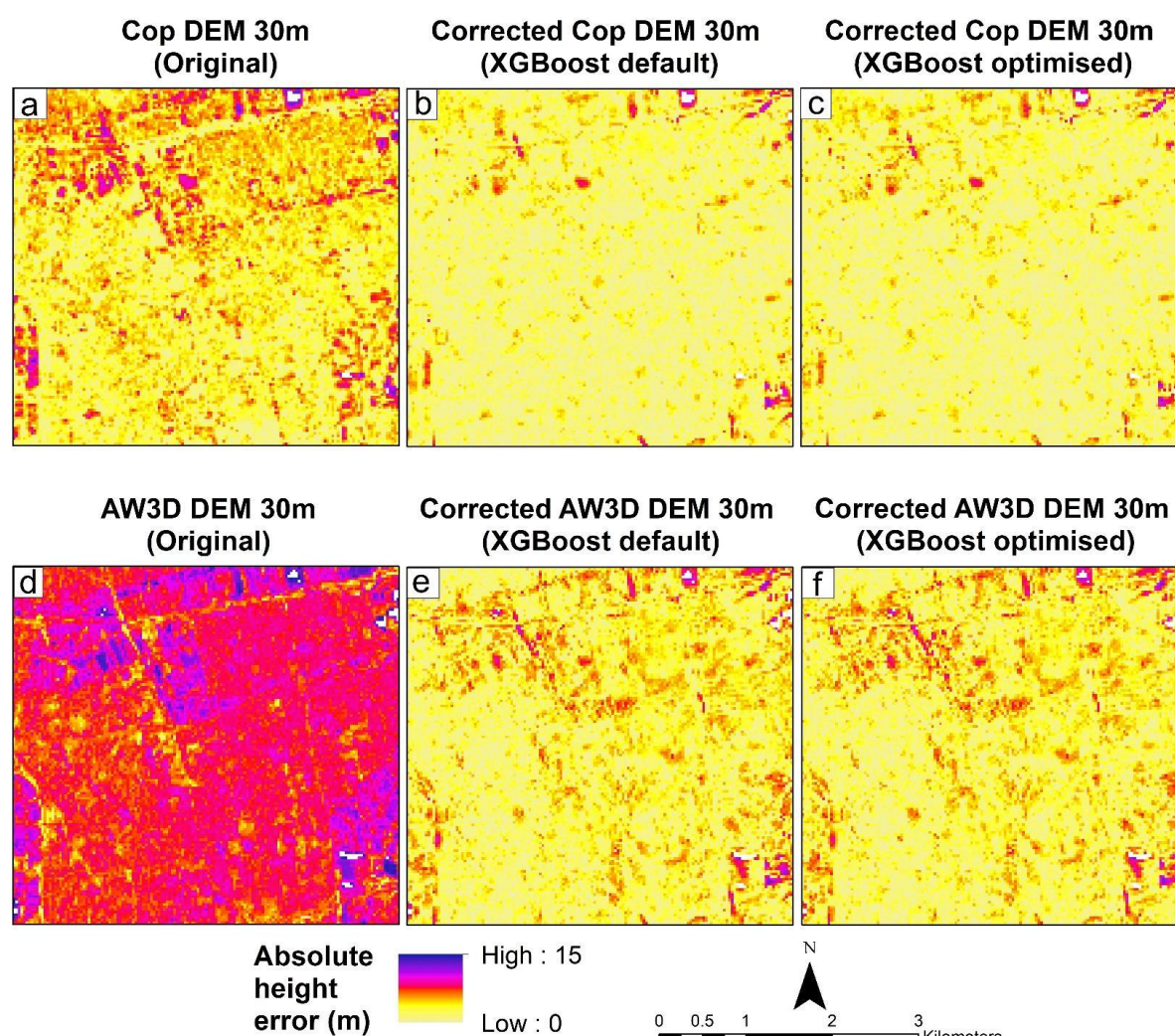
Figure 4. Height error maps of original vs corrected DEMs at site A, Copernicus (a – c) and AW3D (d – f)
