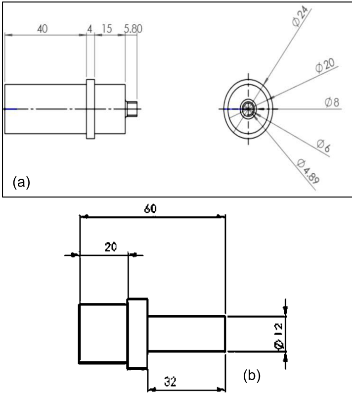
Fig. 1. (a) FSW/FSP tool, and (b) FSP pinless.
