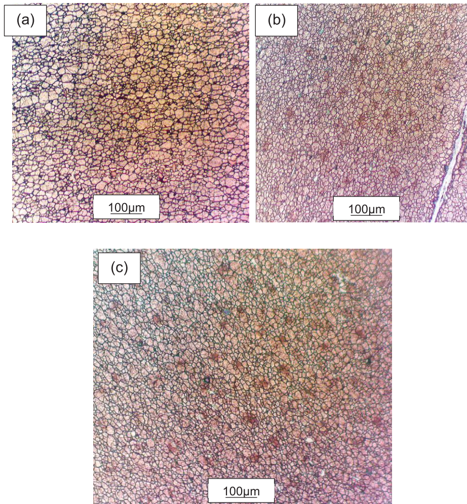
Fig. 6. Stir zone micrographs, (a) FSW, (b) NFSP, and (c) FSP+Coal.
