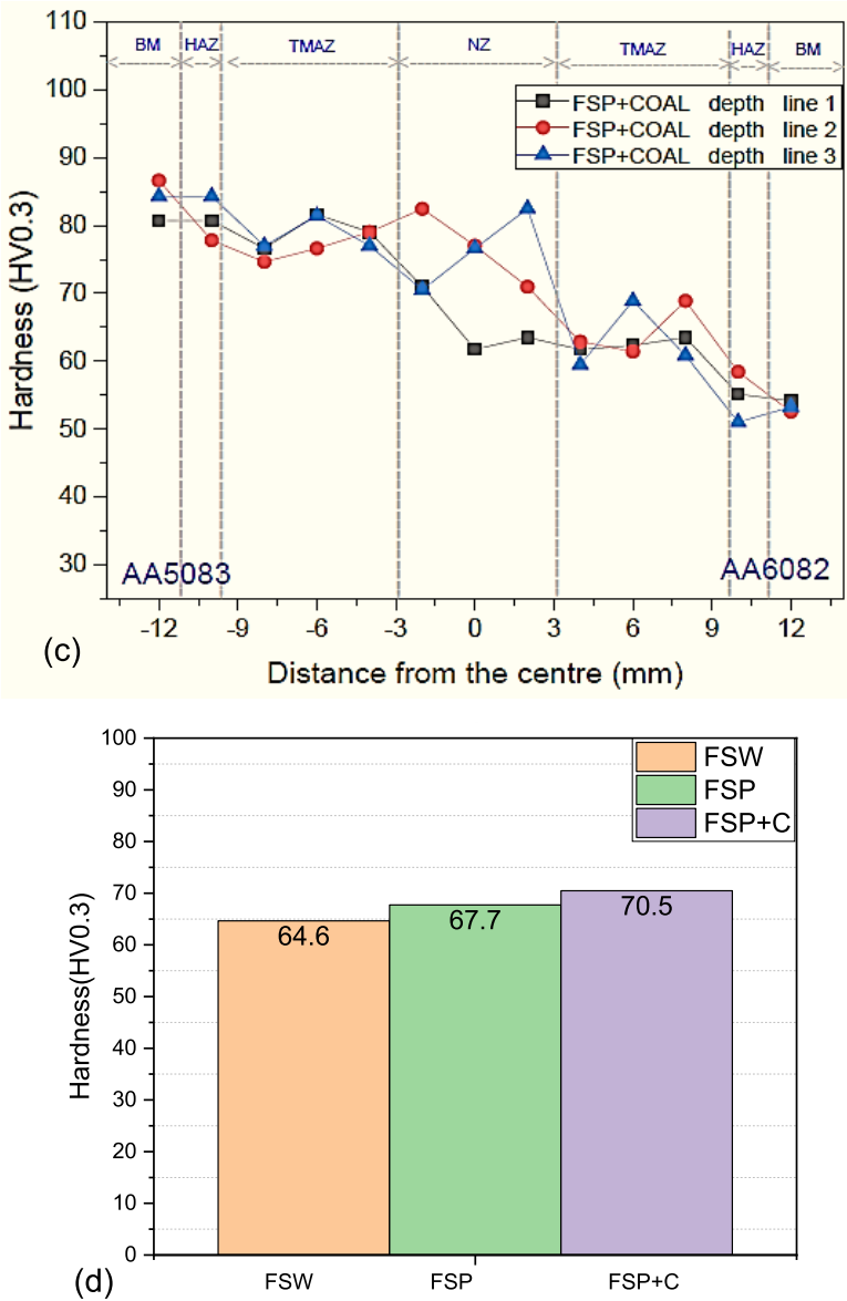
Fig. 9. Microhardness profiles: (a) FSW, (b) FSP, (c) FSP+Coal; (d) Average SZ microhardness charts.
