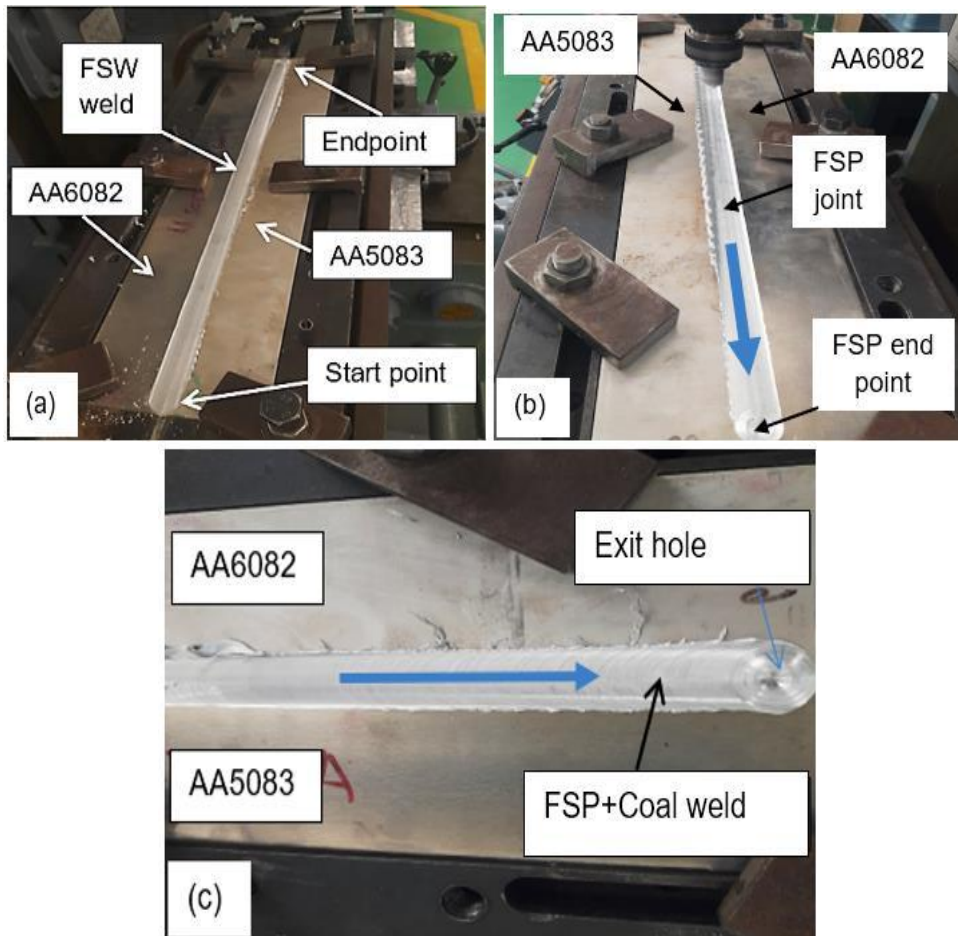
Fig. 3: Produced dissimilar aluminium joints (a) FSW, (b) FSP, and (c) FSP+Coal
