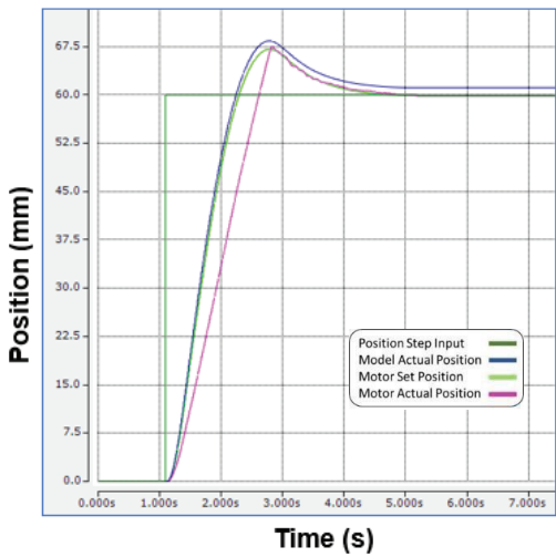
Fig. 10. Step response of 60mm
