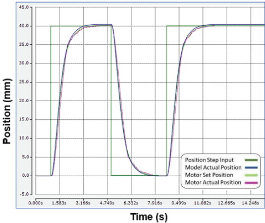
Fig. 9. Step response of 40mm forward and reverse
