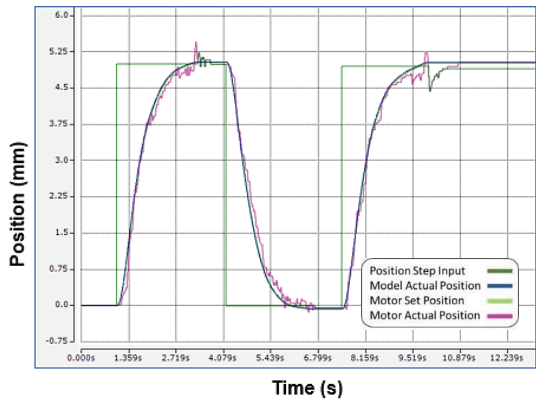
Fig. 8. Step response of 5mm forward and reverse
