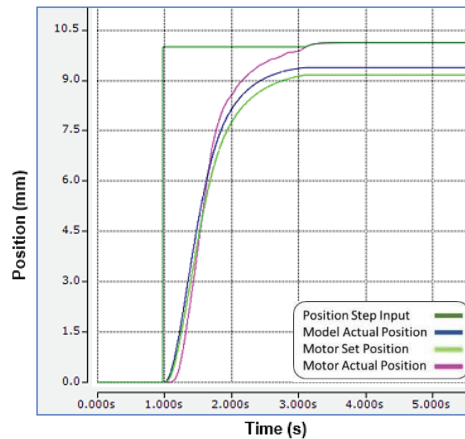
Fig. 5. Step response of 10mm without time delay compensation
