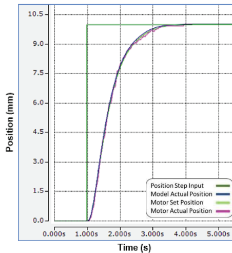
Fig. 7. Step response of 10mm with time delay compensation
