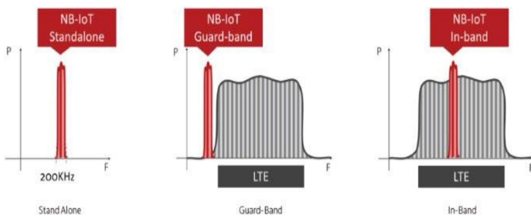
Figure 1. NB-IoT three deployment modes. (Source: Tian & Wang, 2020 )
