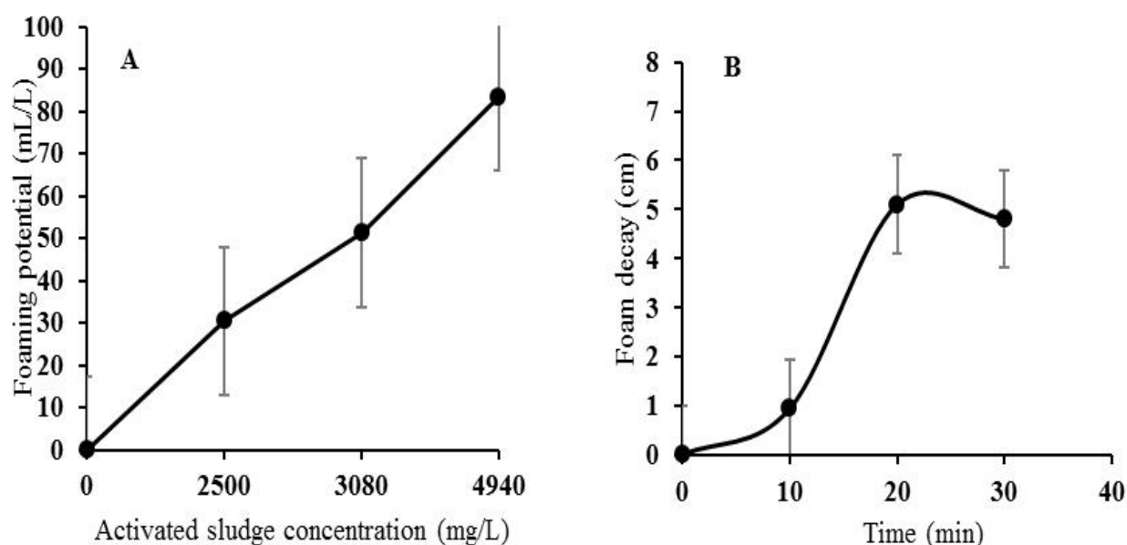
Figure 2. (A) The effect of activated sludge concentration on foaming potential; (B) biofoam decay rate.
