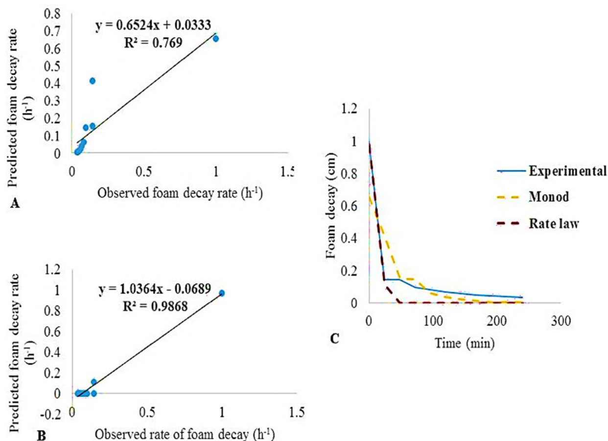
Figure 3. Consistency plots of (A) Monod's model, (B) the rate law, and (C) illustration of the model plots in comparison to experimental foam decay data.
