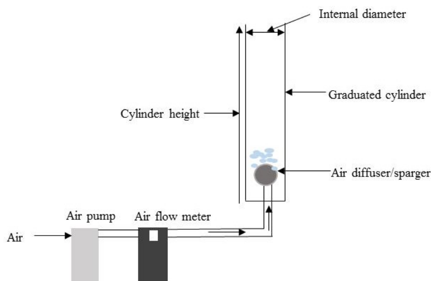
Figure 1. Foaming apparatus setup.
