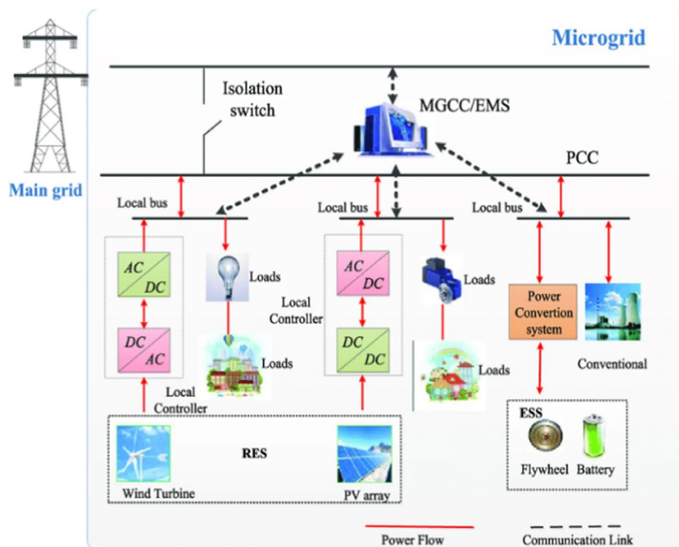
Fig. 2 Micro-grid architecture [24]
