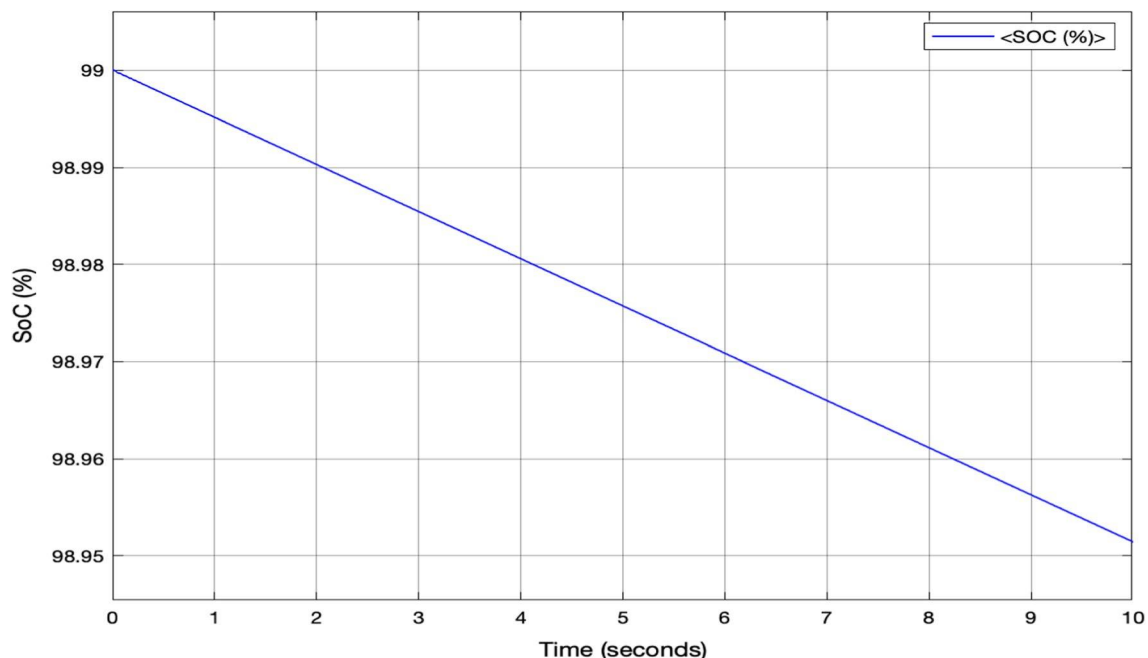
Fig. 12 Battery discharging
