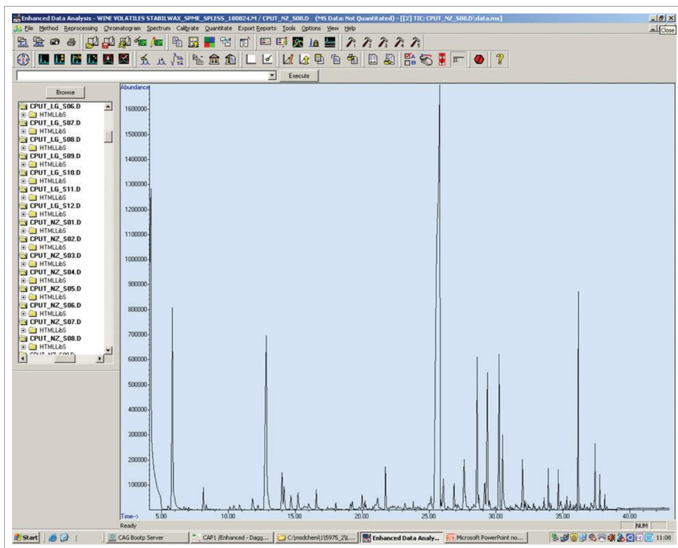
FIGURE 4: Chromatogram for H.cymosum aquaponics plants (T1).
