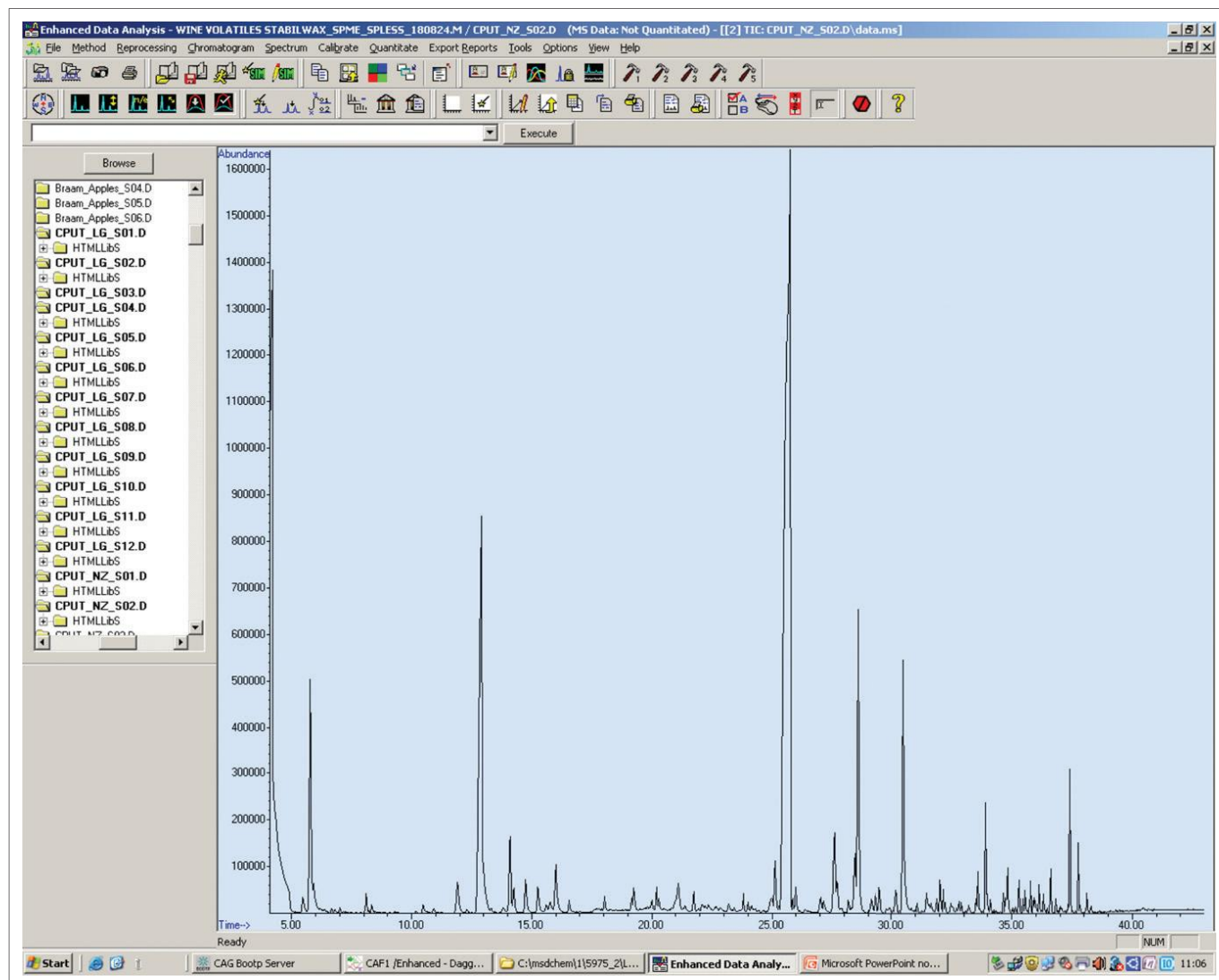
FIGURE 2: Chromatogram for H. cymosum field plants (T3).
