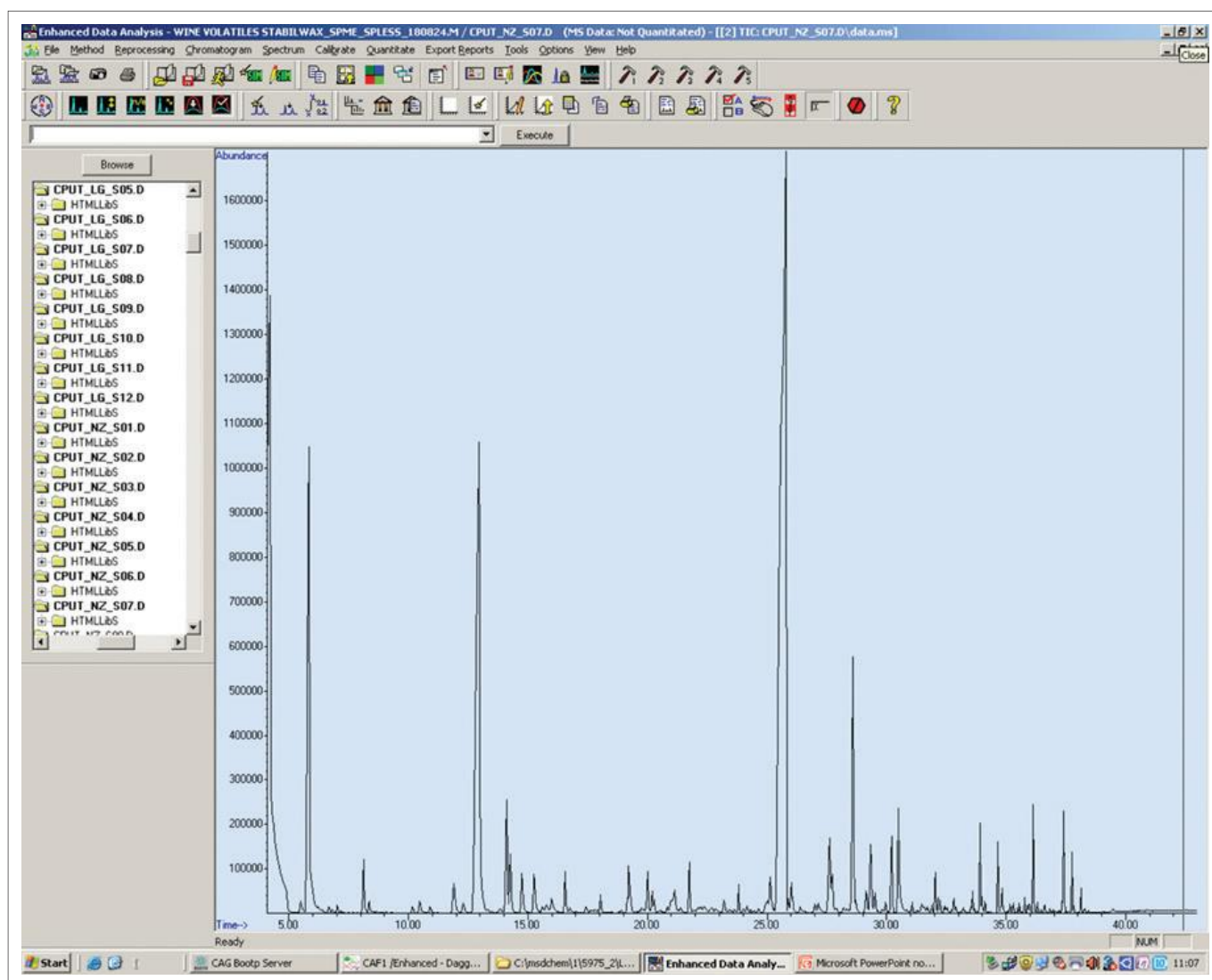
FIGURE 3: Chromatogram for H. cymosum aquaponics plants (T1).
