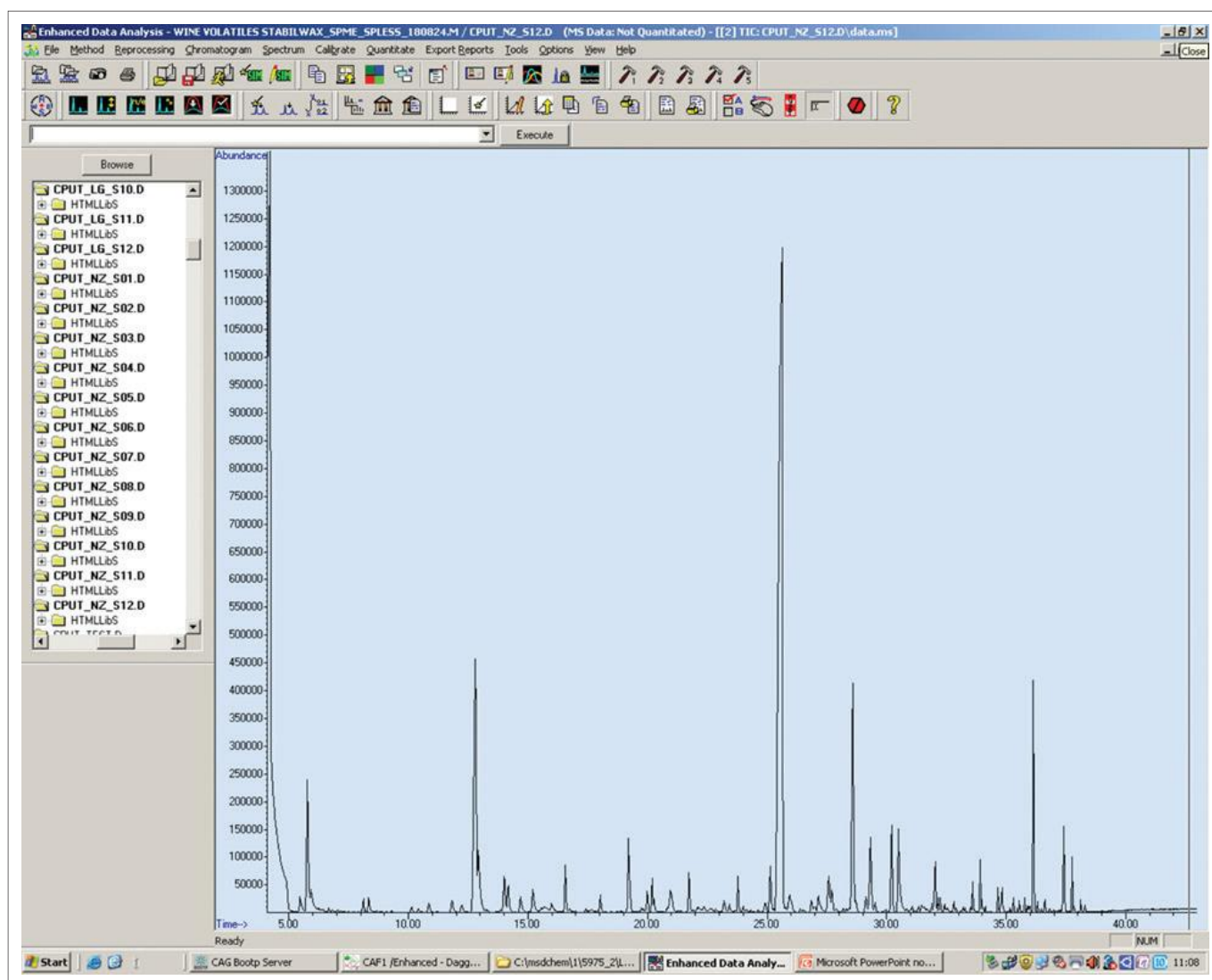
FIGURE 6: Chromatogram for H. cymosum hydroponics plants (T2).
