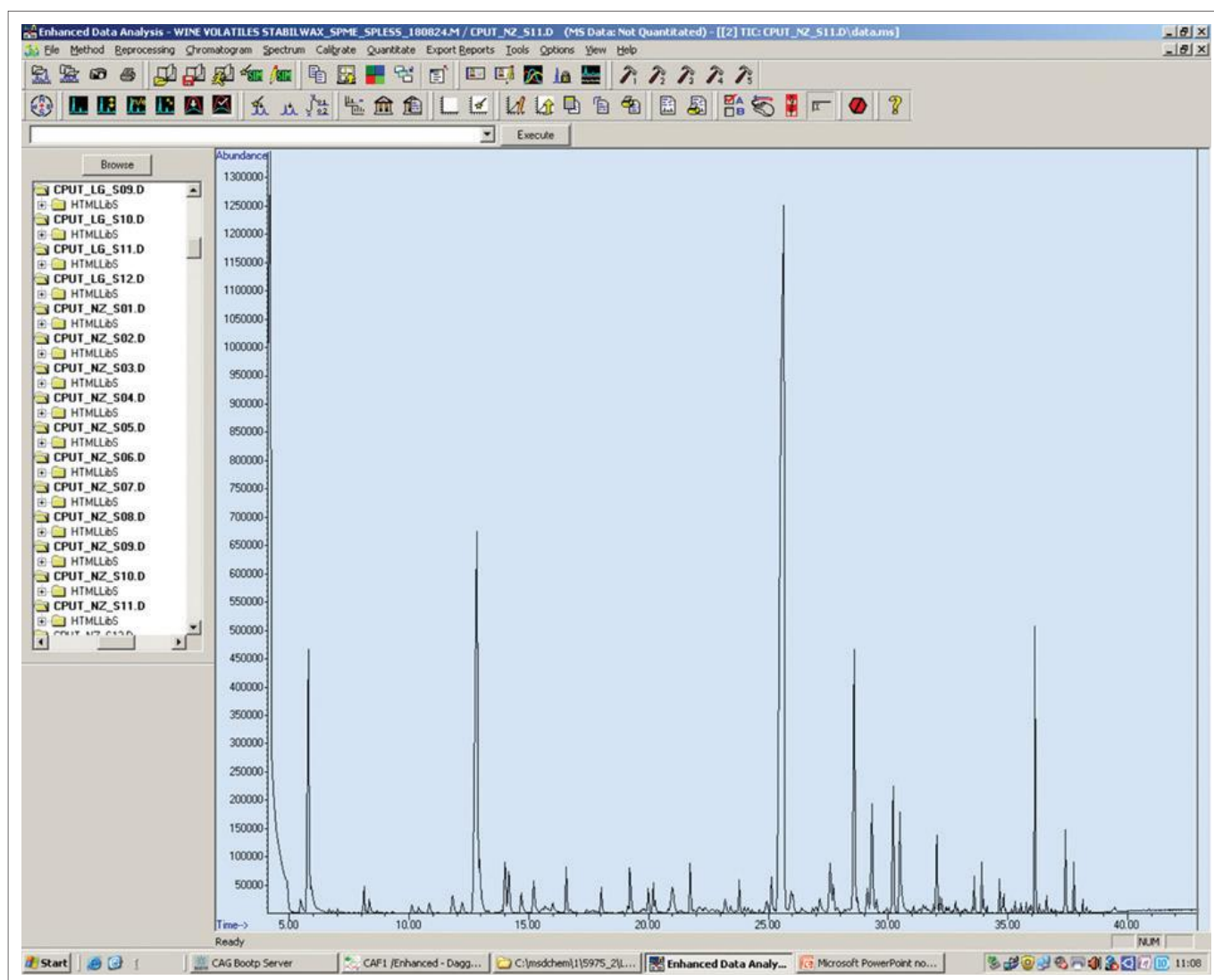
FIGURE 5: Chromatogram for H. cymosum hydroponics plants (T2).
