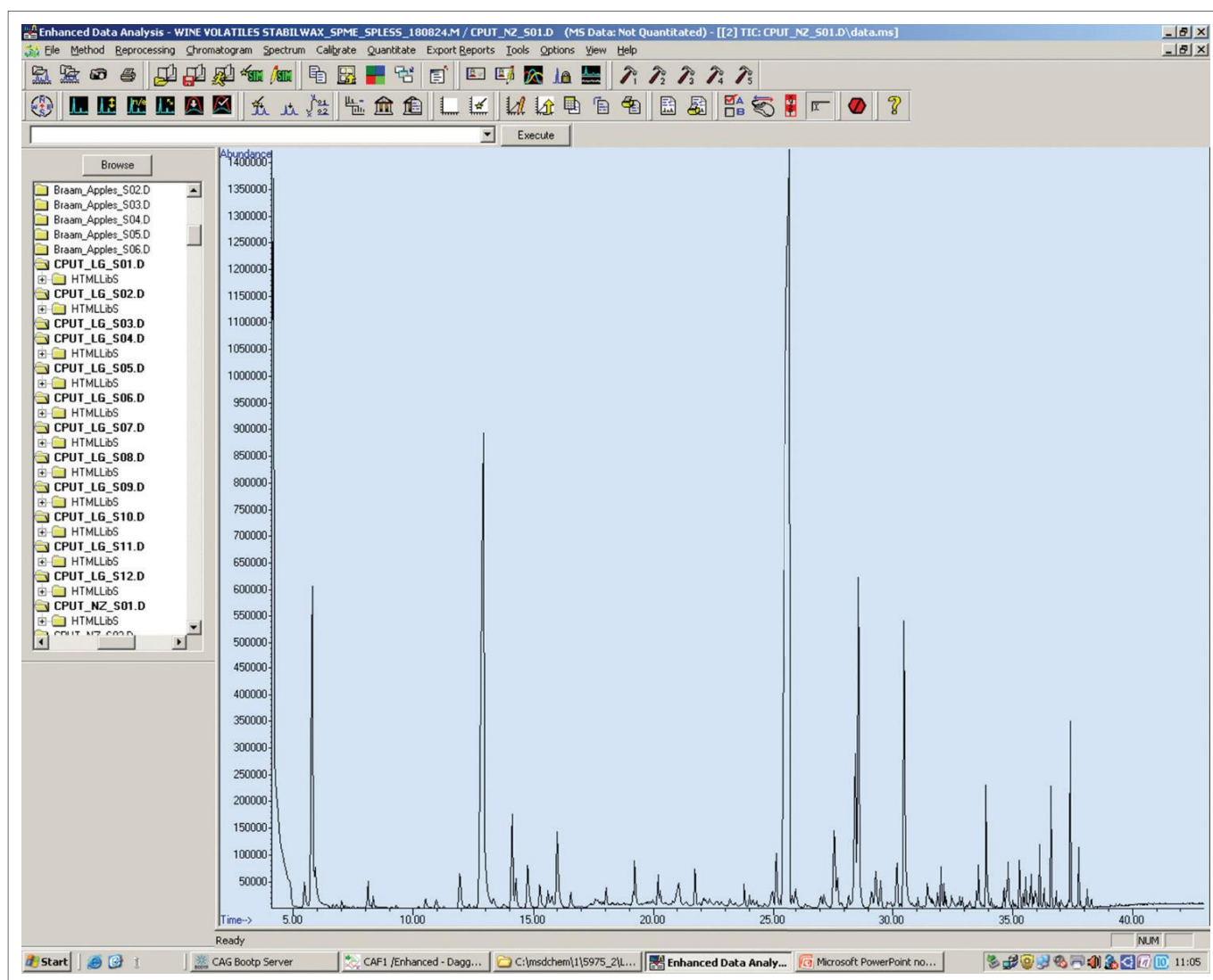
FIGURE 1: Chromatogram for H. cymosum field plants (T3).
