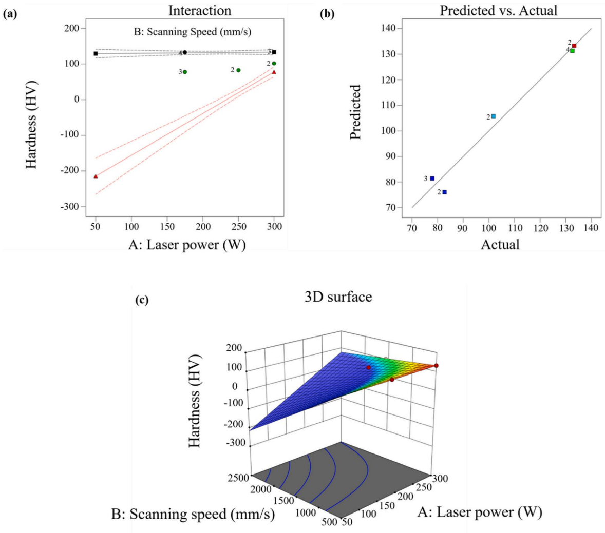
Fig. 9. Interaction of variants with hardness; (a) all factors; (b) predicted vs. actual plot; (c) contour plot.
