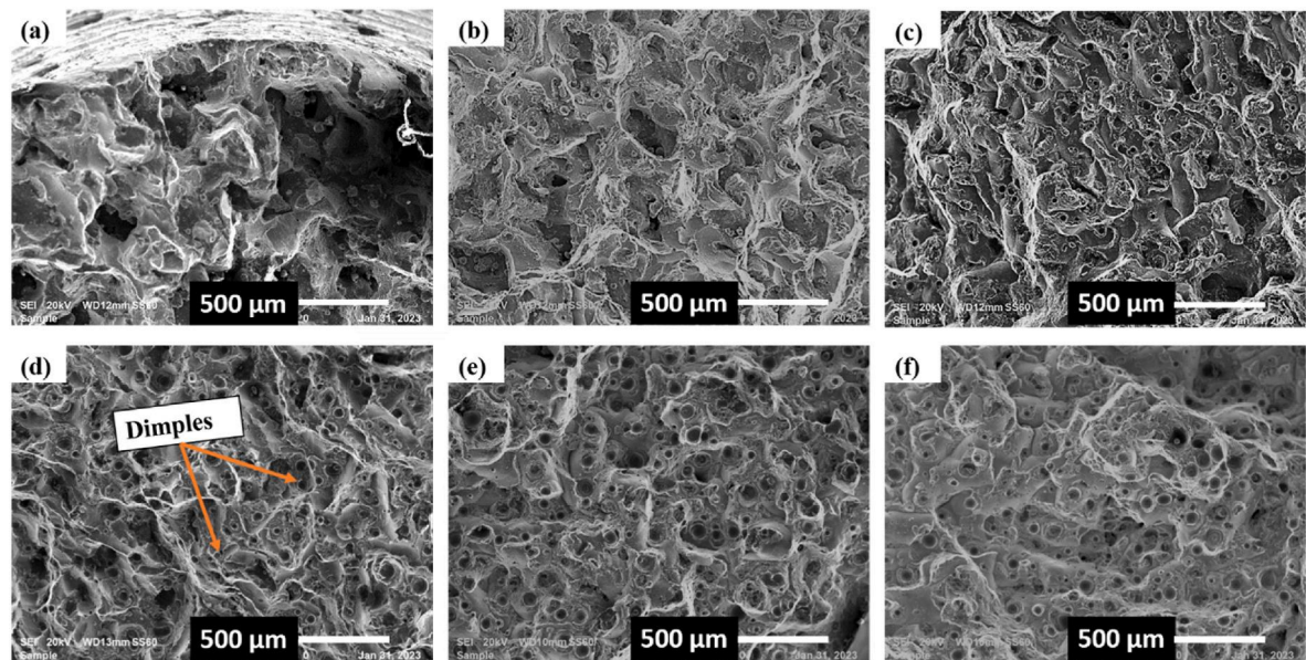
Fig. 6. SEM images of the fractured surface of batch 2 at different laser powers (W). (a) A: 175 W; (b) B: 200 W; (c) C: 225 W; (d) D: 250 W; (e) E: 275 W; (f) F: 300 W.
