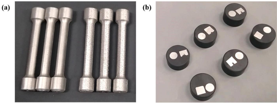
Fig. 1. Tensile specimens; (b) cross-sectional mounted specimens.
