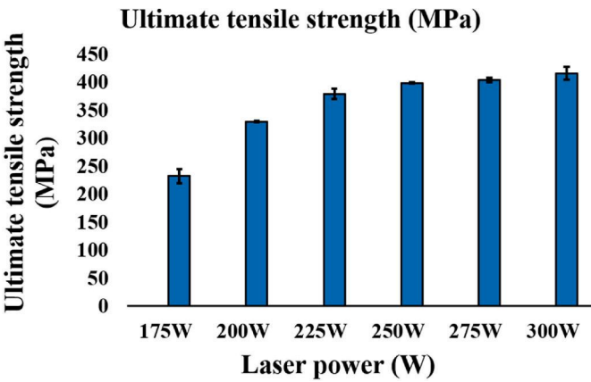
Fig. 12. Ultimate tensile strength results from batch 2.
