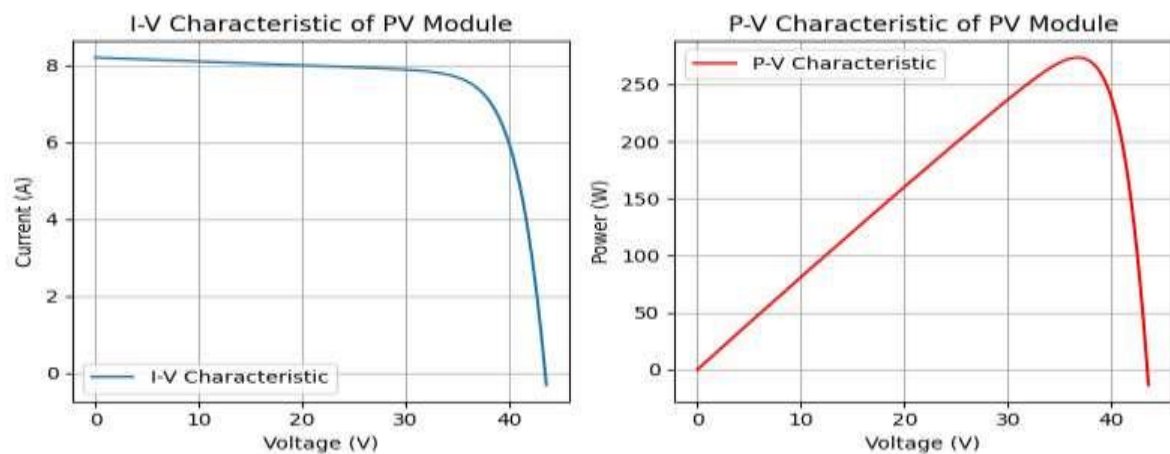
Figure 4: I-V Characteristics
