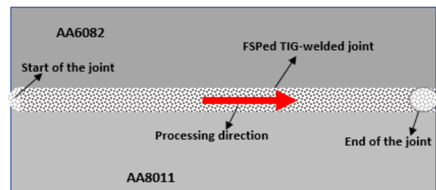
Fig. 2. Schematic diagram of the friction stir processed TIG-welded plate.
