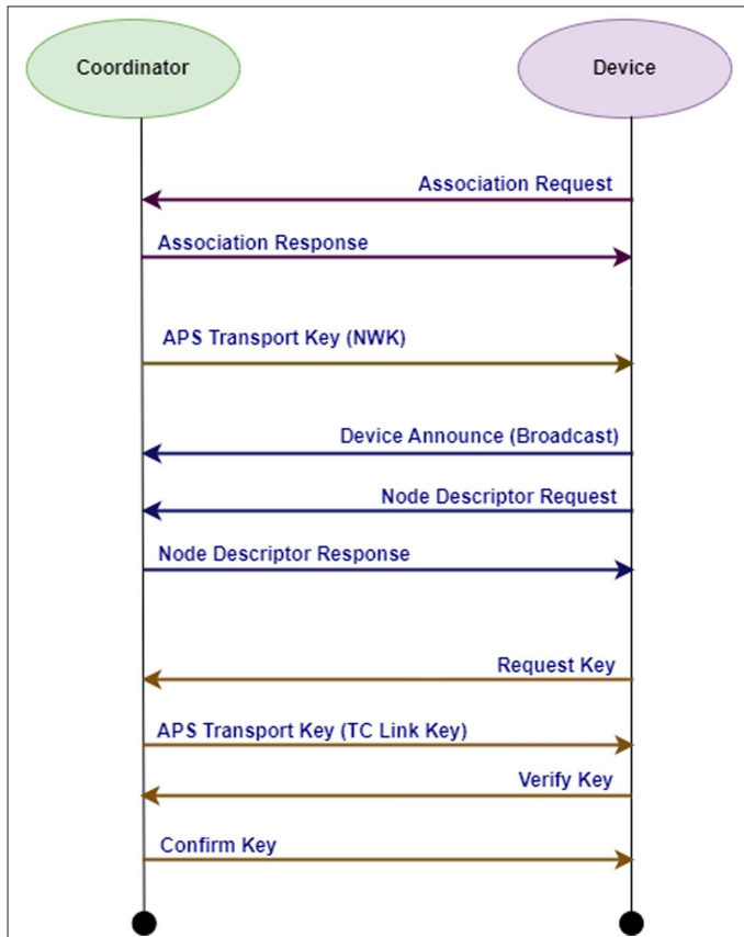
Fig. 2. Joining procedure.
