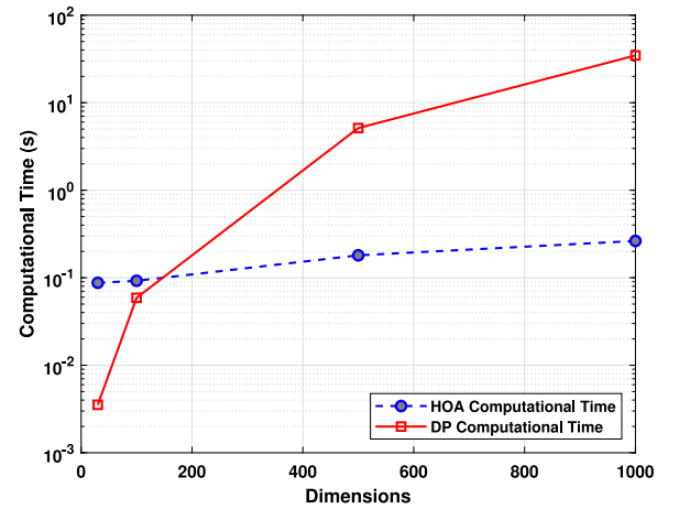
Fig. 8. Computational running time of HOA and DP in solving a 0–1 knapsack problem for varying dimensions of 30, 100, 500, and 1000.
