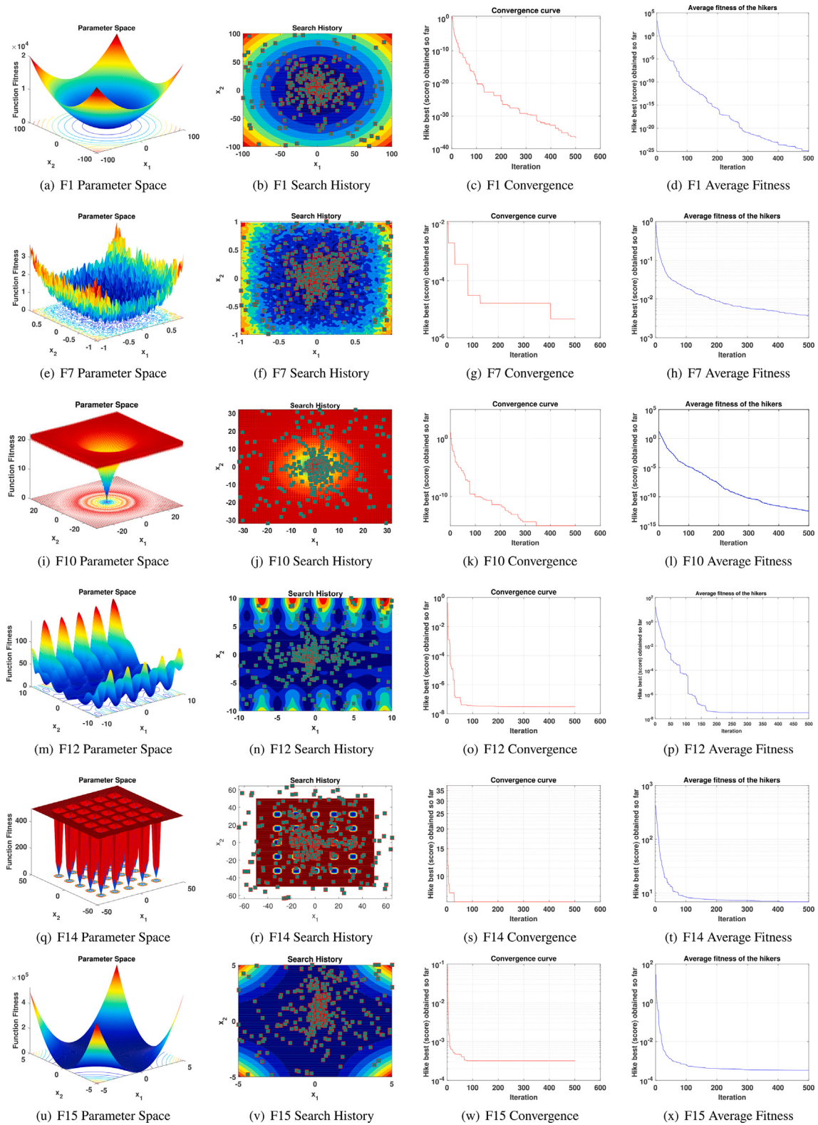
Fig. 9. Illustration of the parameter space, HOA's search, convergence, and fitness average analysis for some functions.
