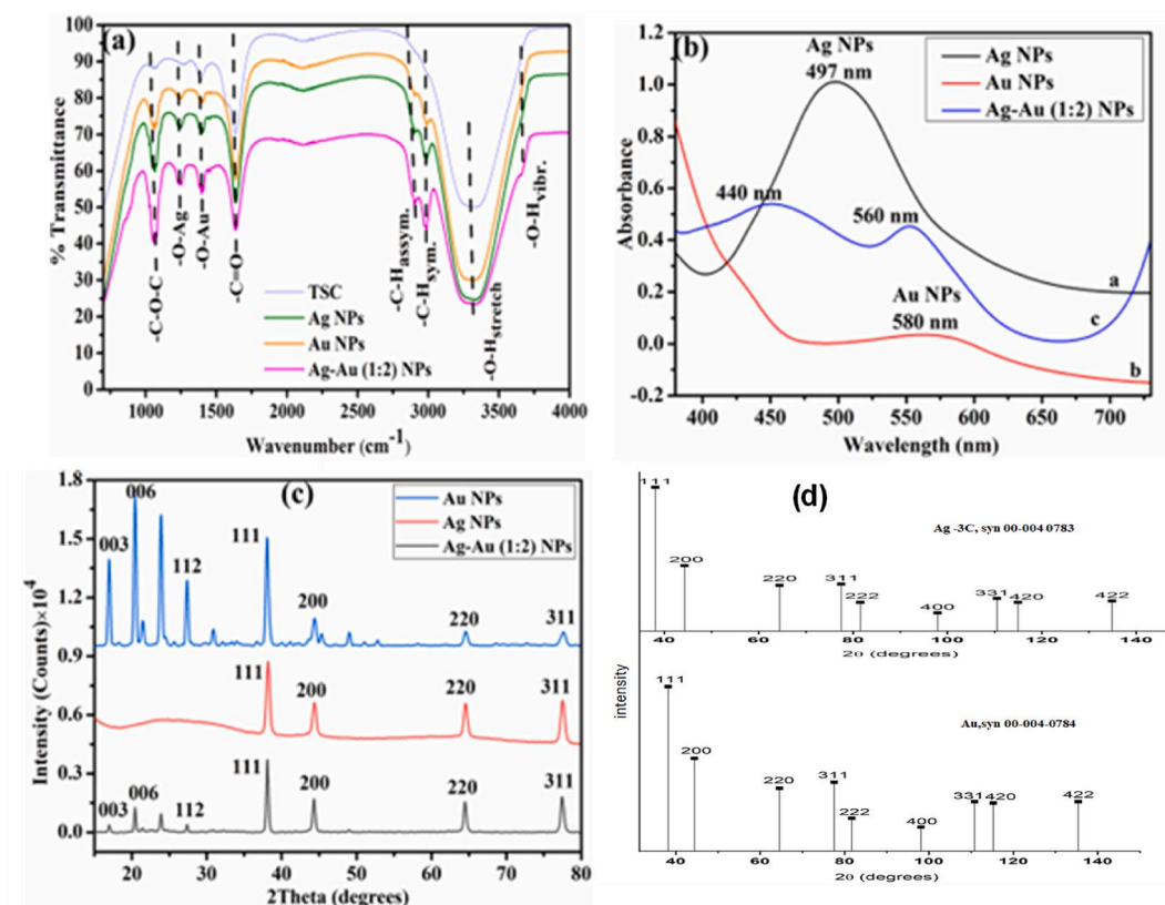
Fig. 1. An overlay spectra of chemically Synthesized Ag NPs, Au NPs and Ag-Au (1:2) NPs; (a) FT-IR, (b) UV-visible and (c) XRD and (d) JPDS spectra.
