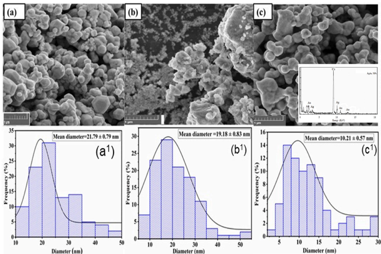
Fig. 2. Scanning electron micrographs of (a) Ag NPs, (b) Au NPs and (c) Ag-Au (1:2) bimetallic NPs with their corresponding diameter histograms; (a'), (b') and (c') respectively.
