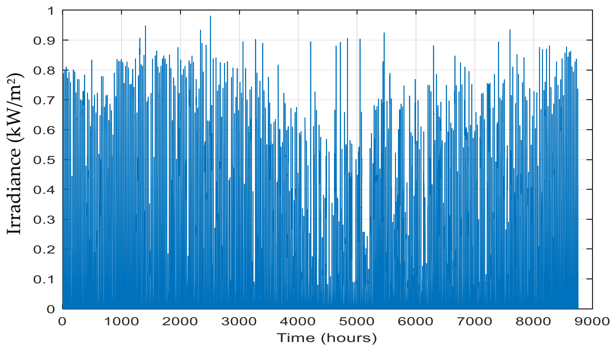
Figure 3. Solar irradiance hourly profile.
