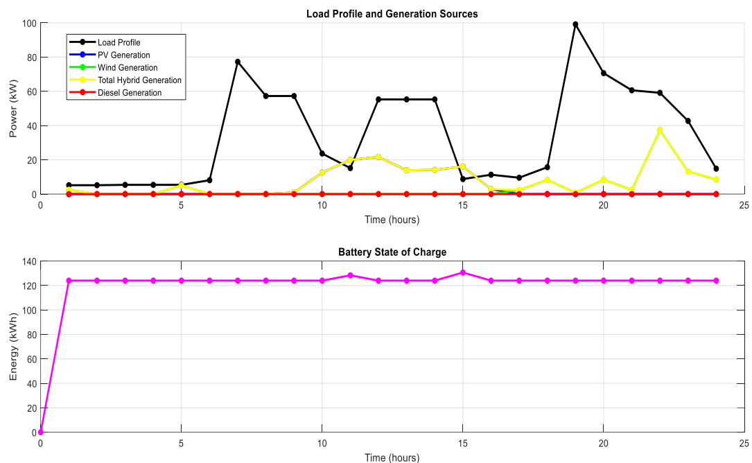
Figure 16. Case 2 performance.
