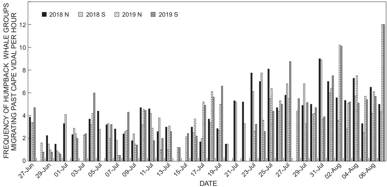
Figure 4: Daily number of humpback whale groups migrating per hour past Cape Vidal, South Africa, observed from the north (N) and south (S) towers in the 2018 and 2019 surveys
