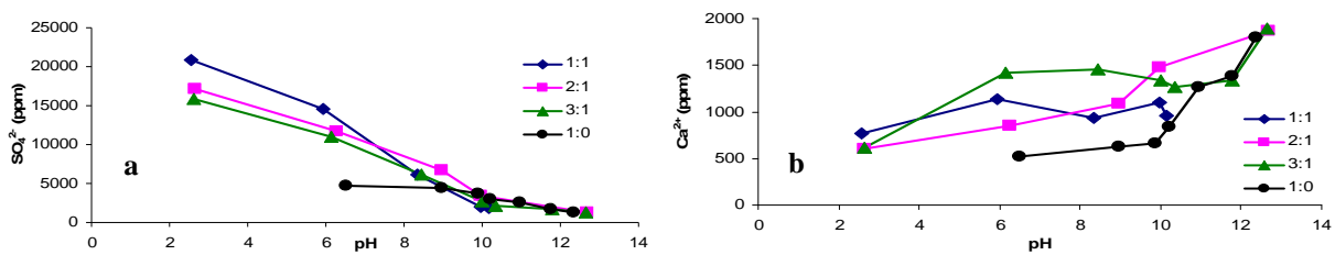
Fig 4. Trends of sulphate (a) and Ca (b) concentrations during treatment of CMW and different CMW:AMD ratios with FA
