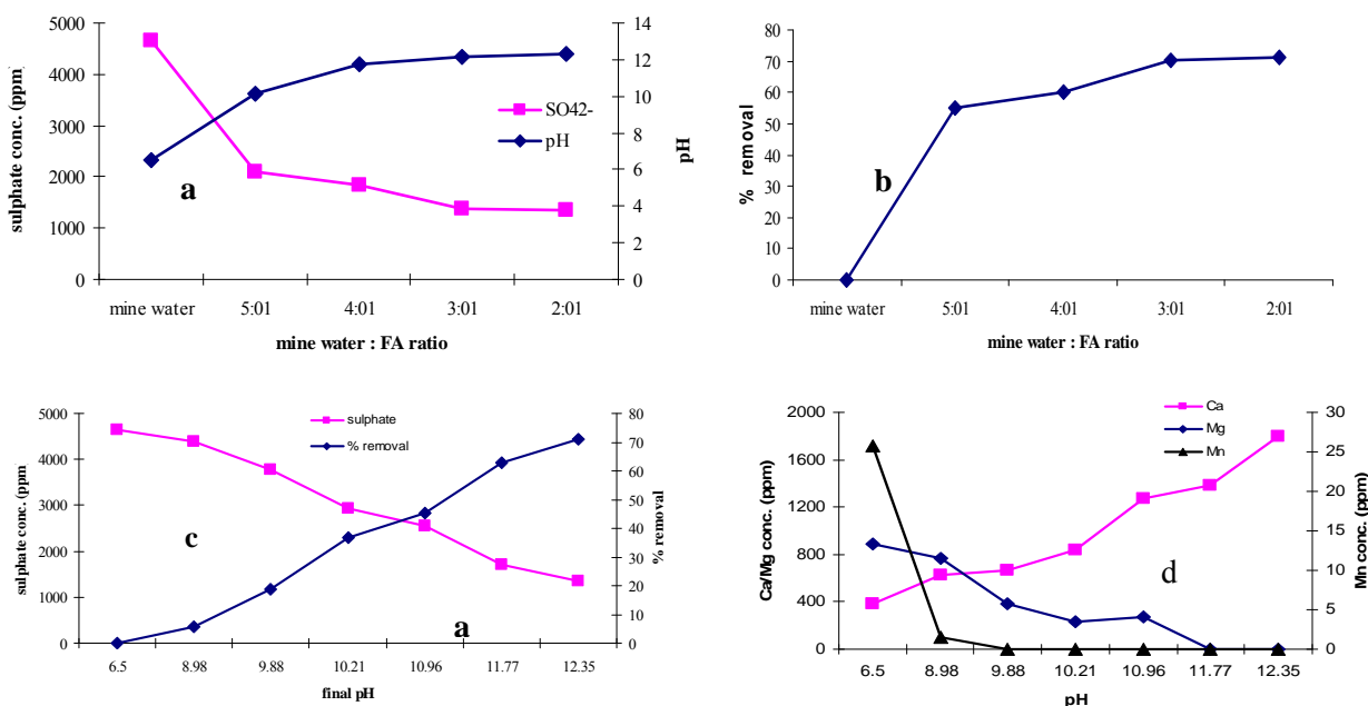
Fig 1. Sulphate concentration during treatment of NMD with different amounts of FA (a), % sulphate removal of sulphates using different amounts of FA (b), % removal of sulphates at different NMD: FA ratios (c) and the Ca/Mg and Mn concentration trends (d) during treatment of NMD to different final pH.
