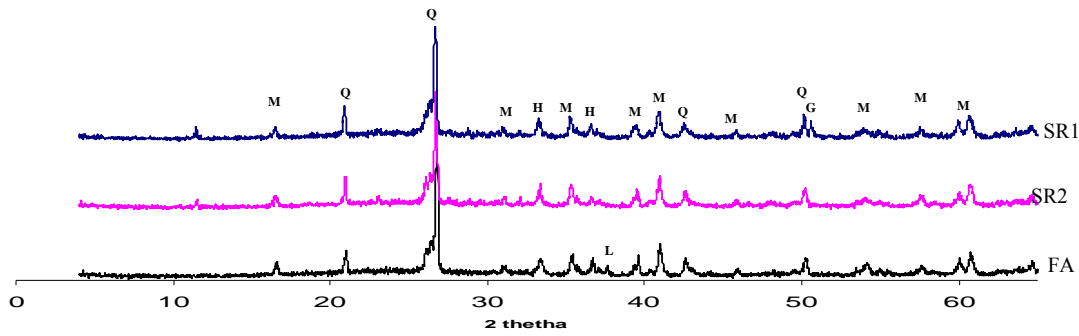
Figure 2. XRD spectra of FA, solid residues (SR1 and SR2) after treatment of CMW with FA.
