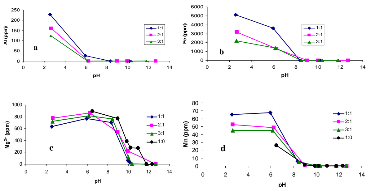
Fig 5. Trends of Al (a), Fe (b), Mg (c) and Mn (d) concentrations during treatment of different CMW and different CMW:AMD ratios with FA.
